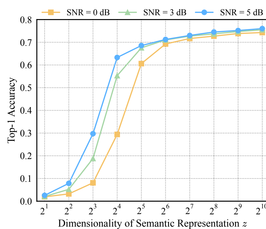
(b) CIFAR-100 / ResNet-34 (conv3_x-conv4_x)
