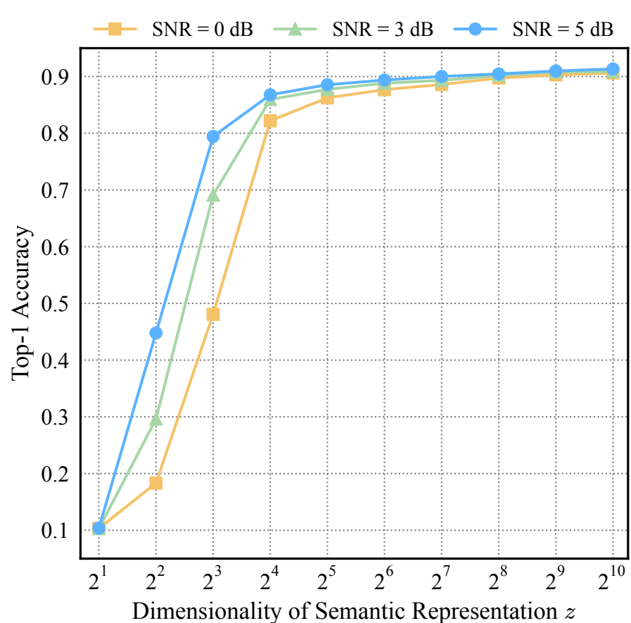
(b) CIFAR-10 / ResNet-34 (conv2_x-conv3_x)
