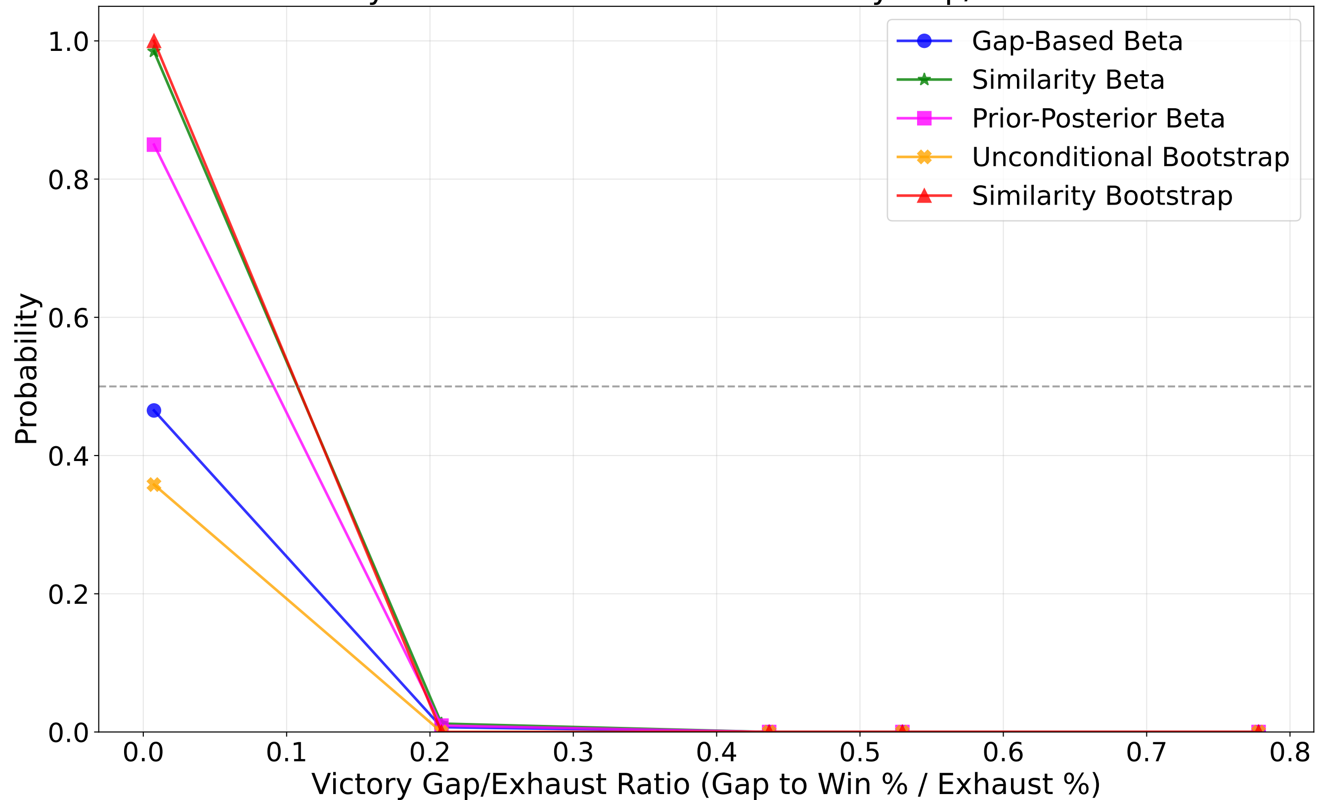
Probability of Alternate Winners Vs Victory Gap/Exhaust Ratio
