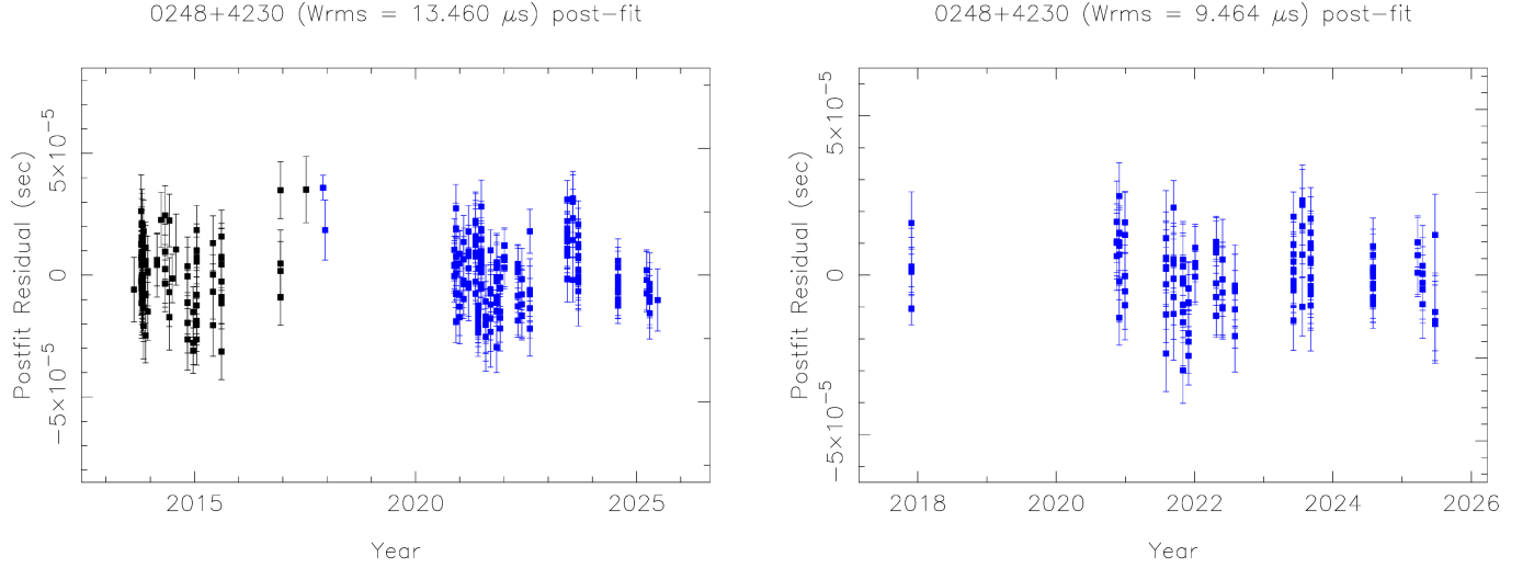
(a) Postfit timing residual from 12 years of timing for PSR J0248+4230 using legacy GMRT and uGMRT observations. Black and Red are data points correspond to band-3 and band-4 observations using legacy GMRT. Blue data points corresponds to band-3 uGMRT observations.
