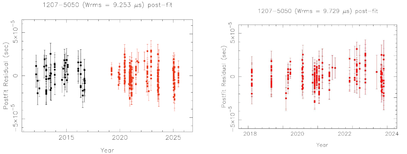
(a) Postfit timing residual from 12 years of timing for PSR J1207-5050 using legacy GMRT and uGMRT observations. Black and Red are data points corresponds band-4 observations using legacy GMRT and uGMRT.
