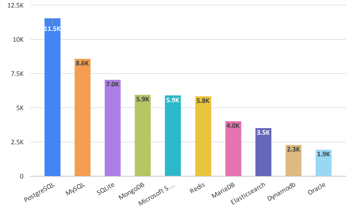
Top 10 Databases Used Current Year
