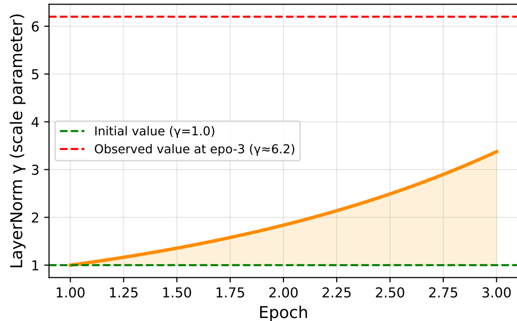
LayerNorm Scale Drift (projection layer)
