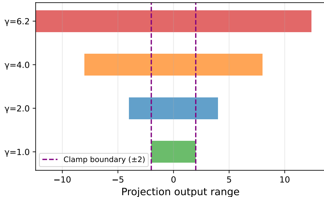
Projection Output Magnitude vs. \gamma value
