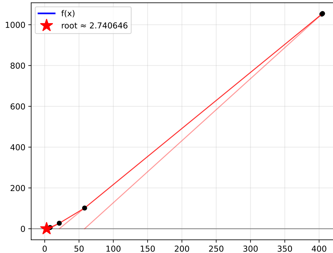
Secant Method (9 iterations)
