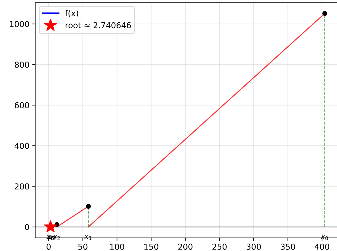
Newton-Raphson (7 iterations)
