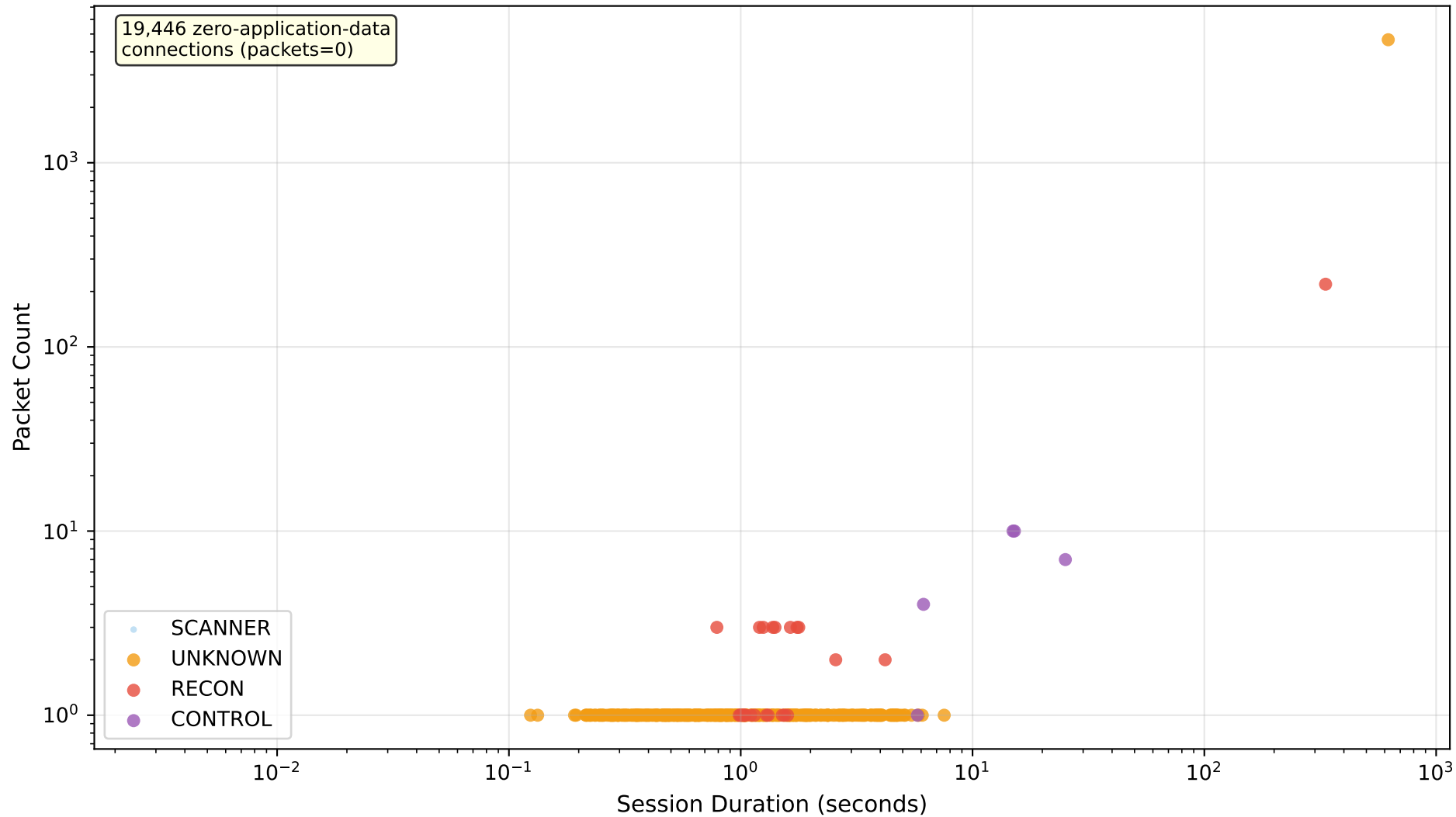
Session Duration vs Packet Count by Intent Class
