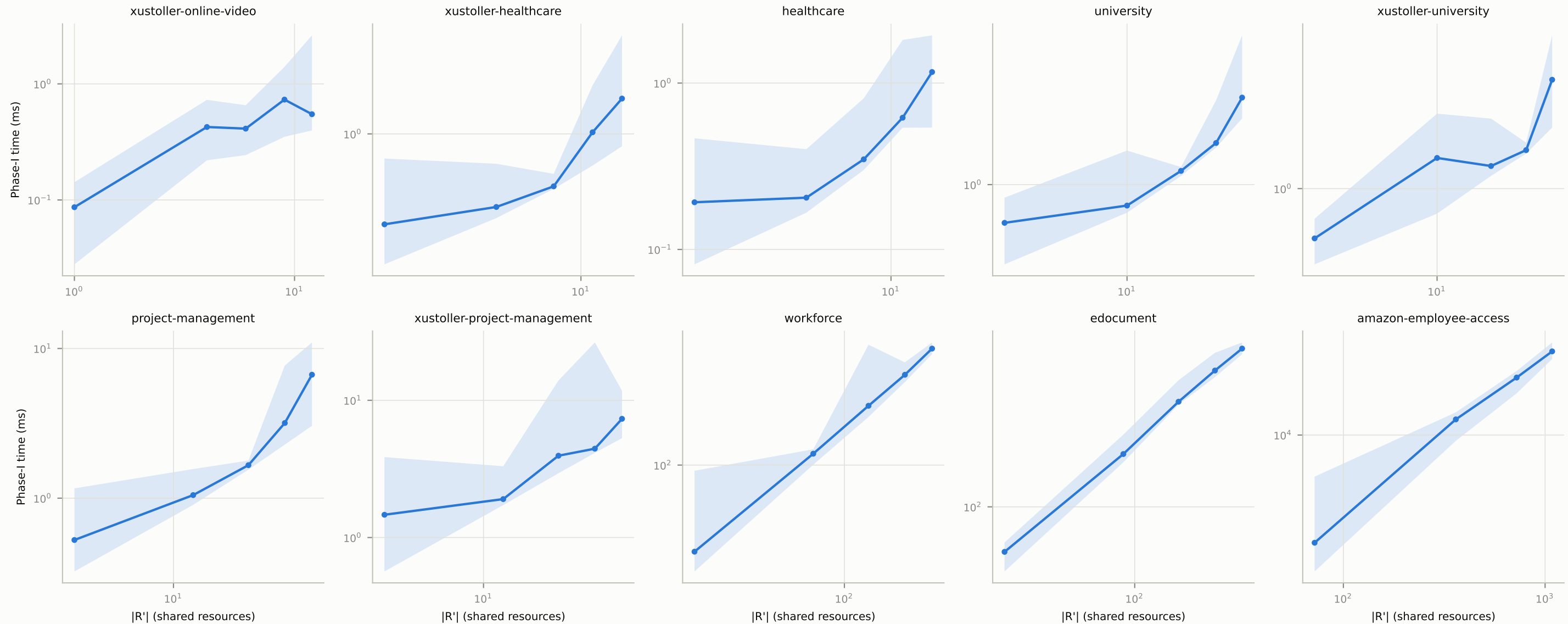
Phase-I runtime vs. shared-resource-set size (median, min-max band over trials, log-log)
