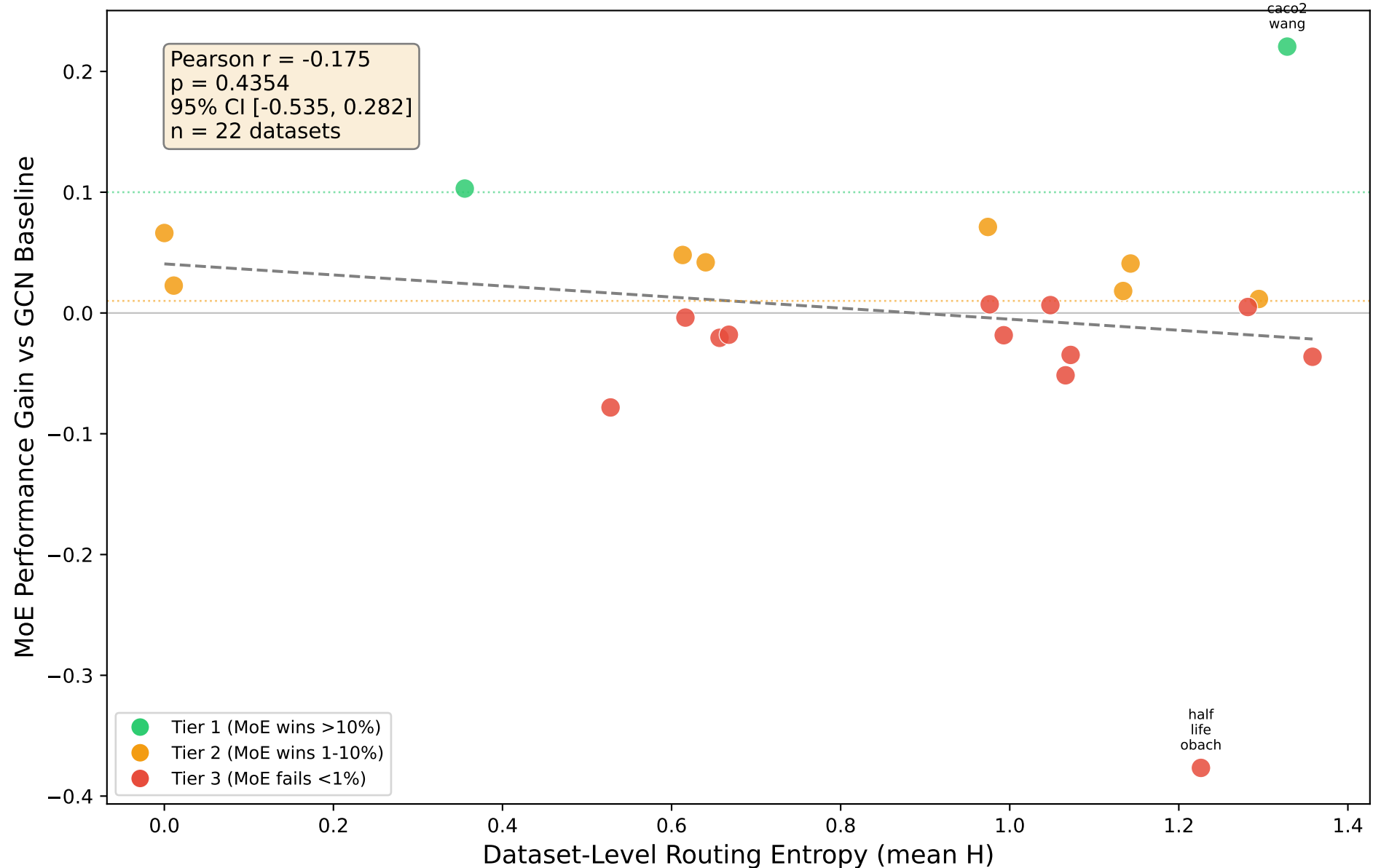
Routing Entropy Predicts MoE Performance Gain Across ADMET Datasets (Lower entropy = stronger chemical cluster structure = larger MoE benefit)
