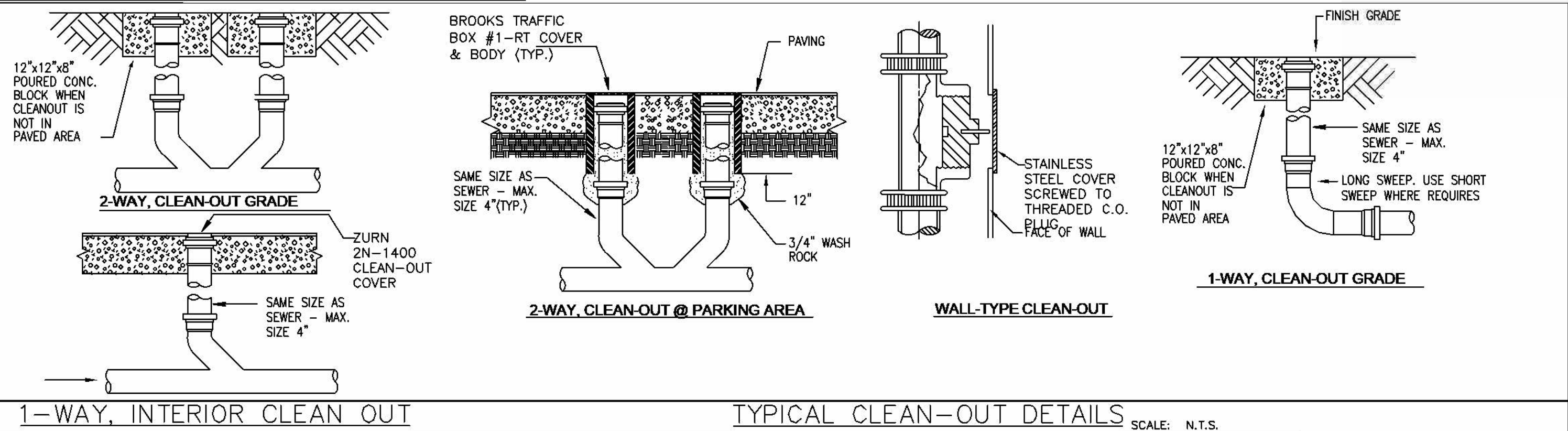
1-WAY, INTERIOR CLEAN OUT
