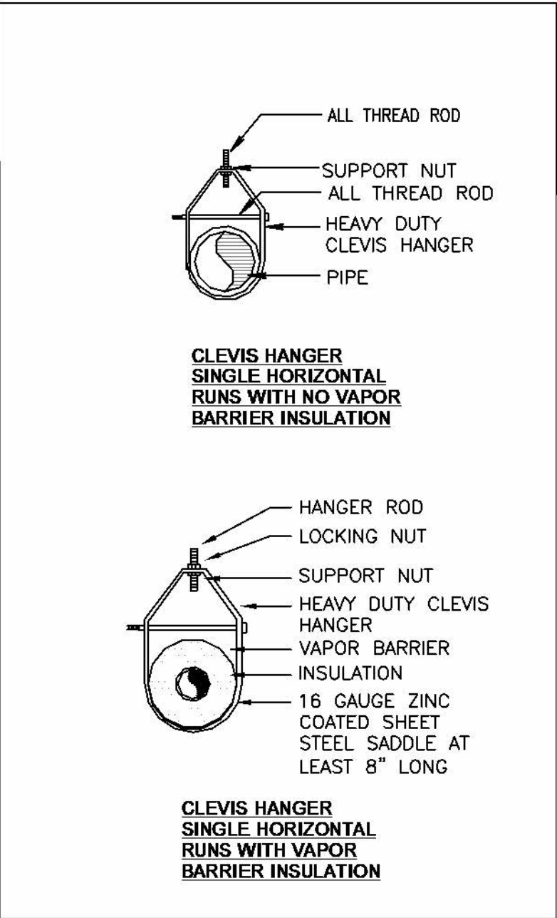
PIPE SUPPORT DETAIL
