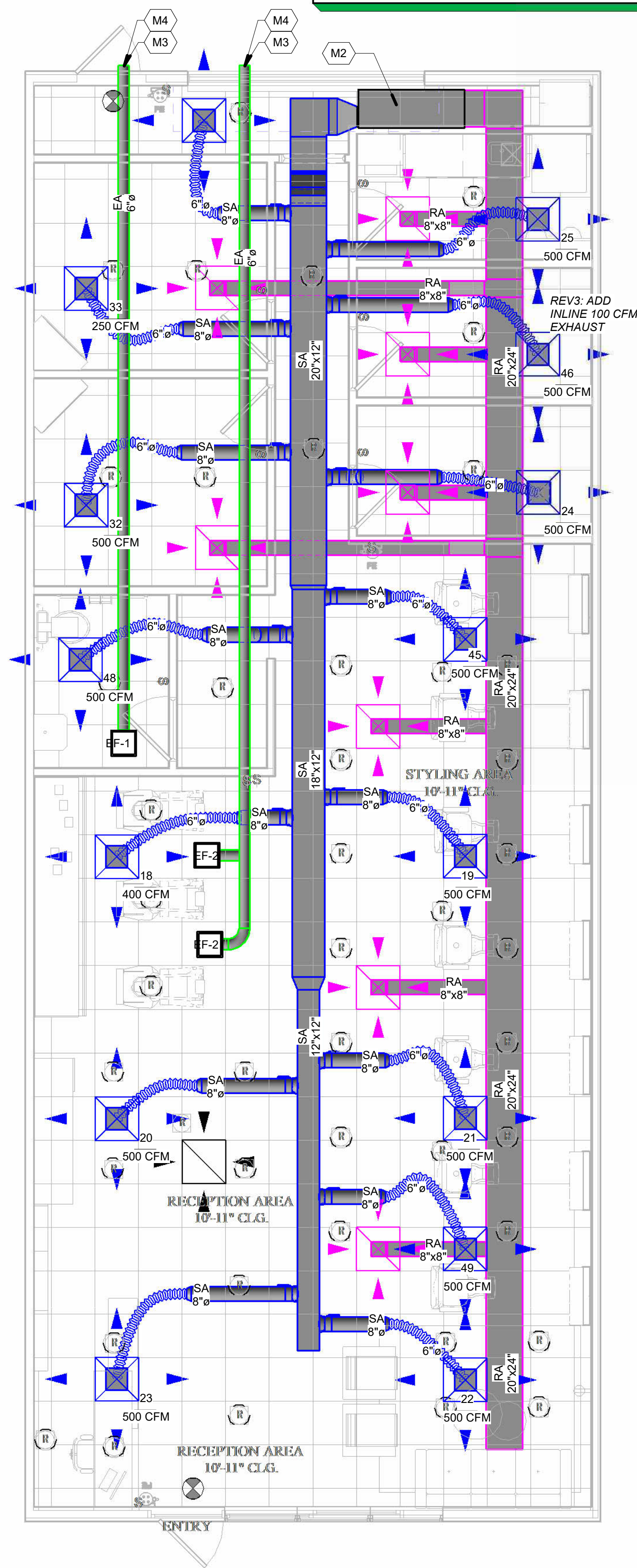
1 PROPOSED MECHANICAL PLAN 1/4" = 1'-0"
