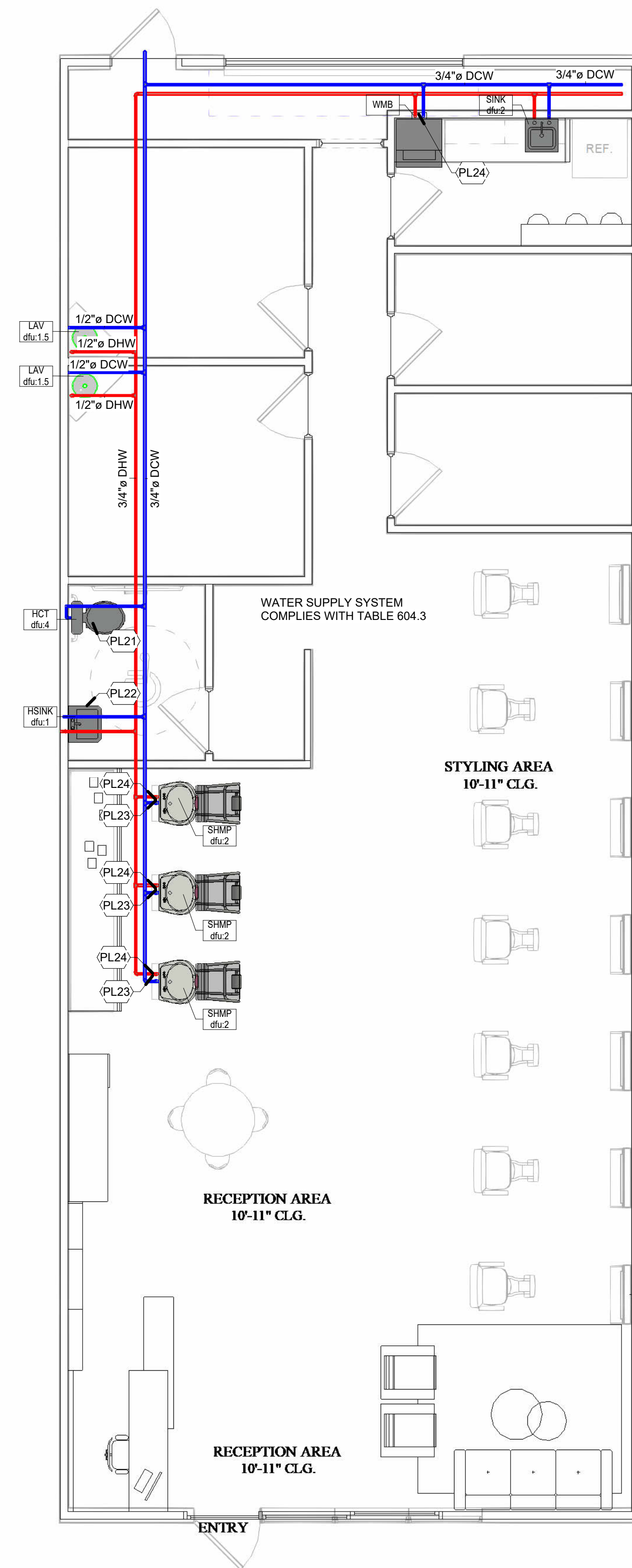
3 PROPOSED WATER DISTRIBUTION PLAN P-1 1/4" = 1'-0"
