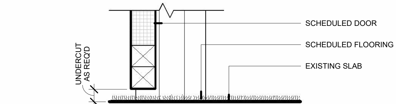
4 SILL @ STANDARD DOOR 3" = 1'-0"
