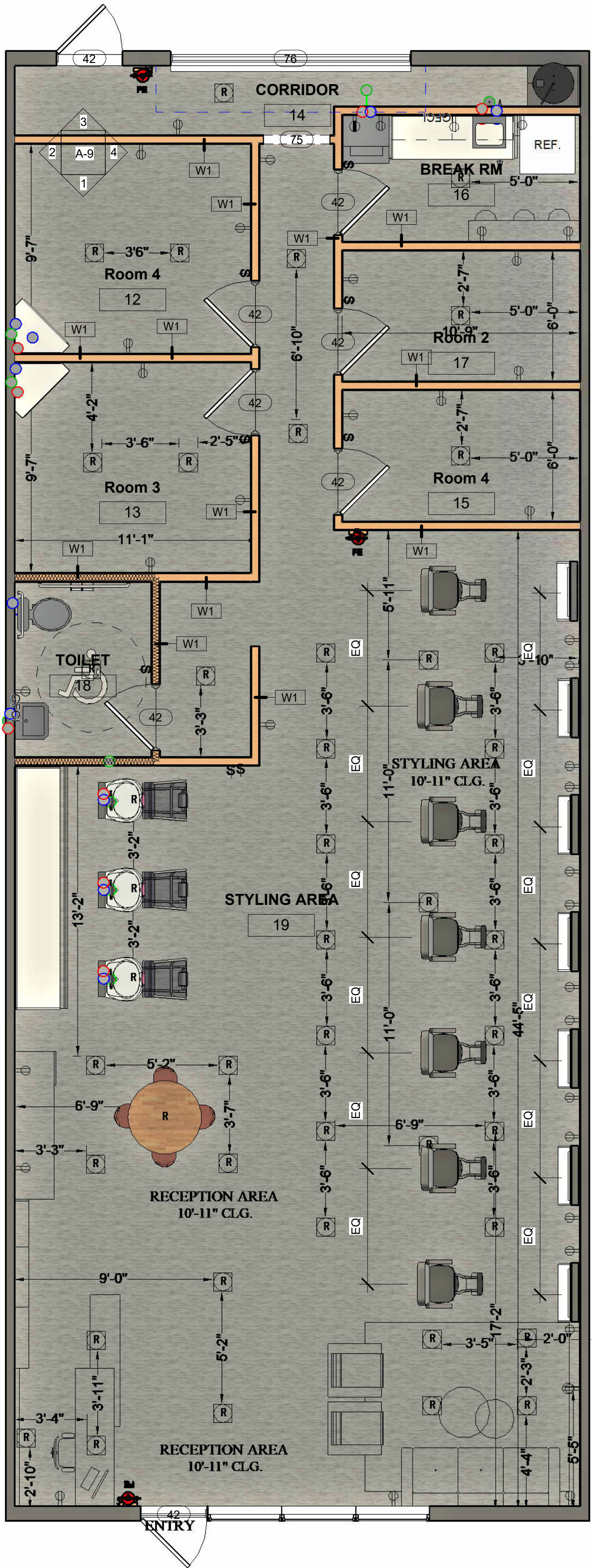
1 FLOOR PLAN 1/4" = 1'-0"
