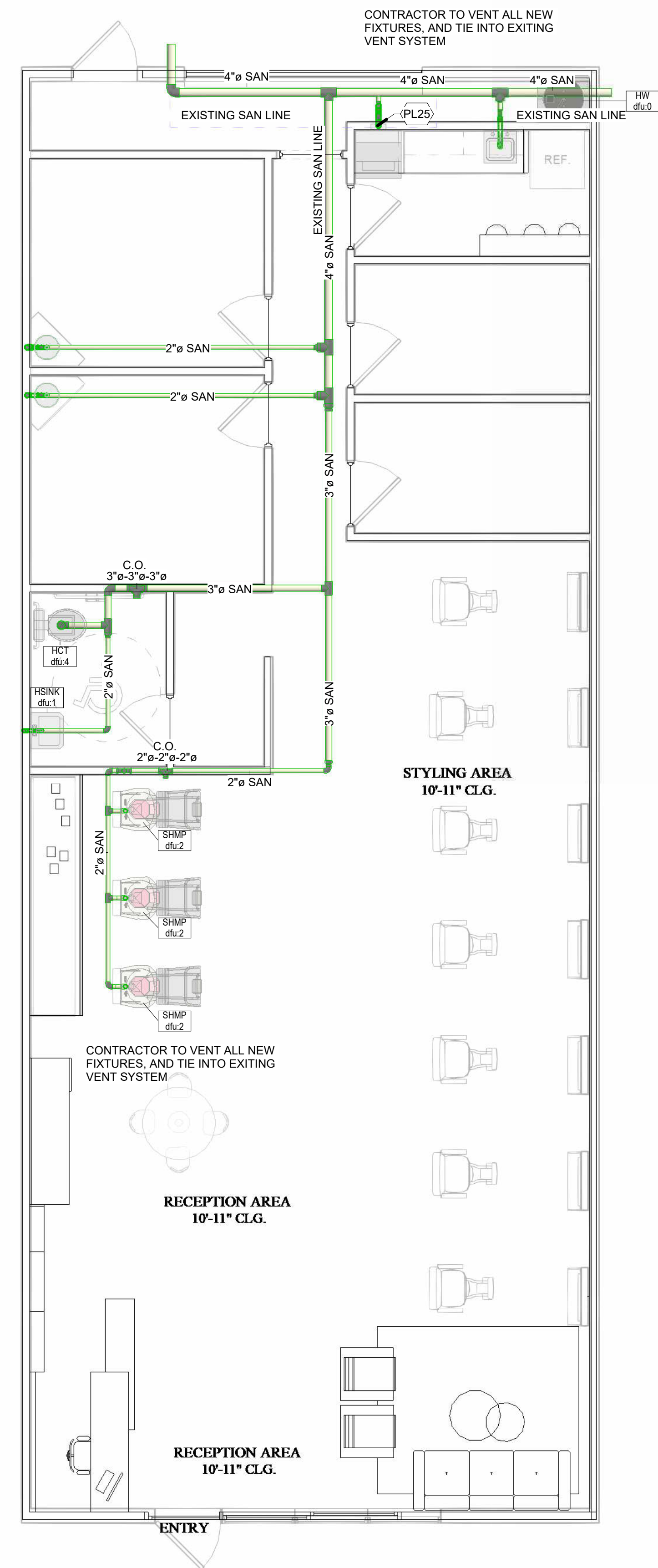
1 PROPOSED PLUMBING PLAN P-1 1/4" = 1'-0"
