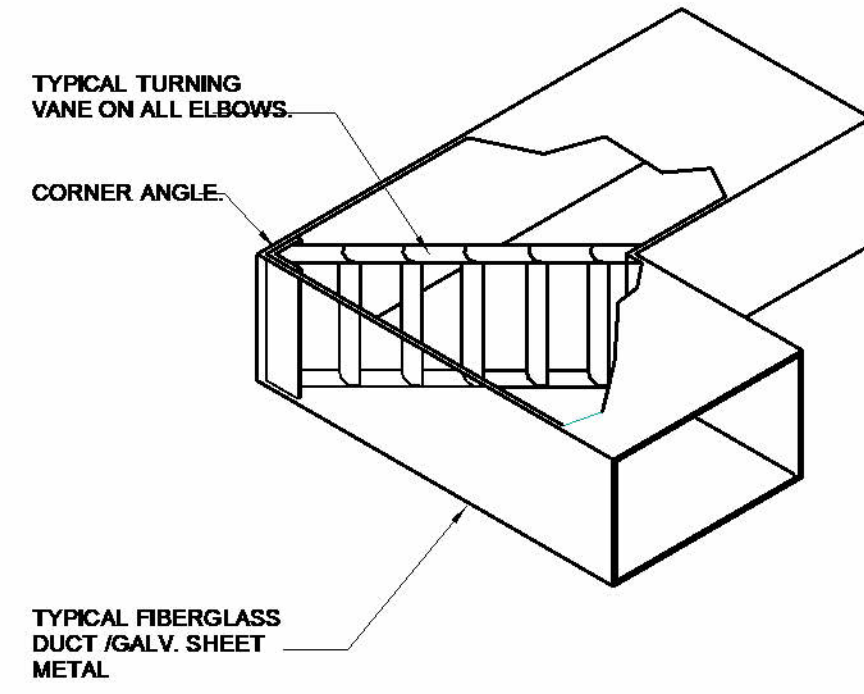
ELBOW TURNING VANE DETAIL
