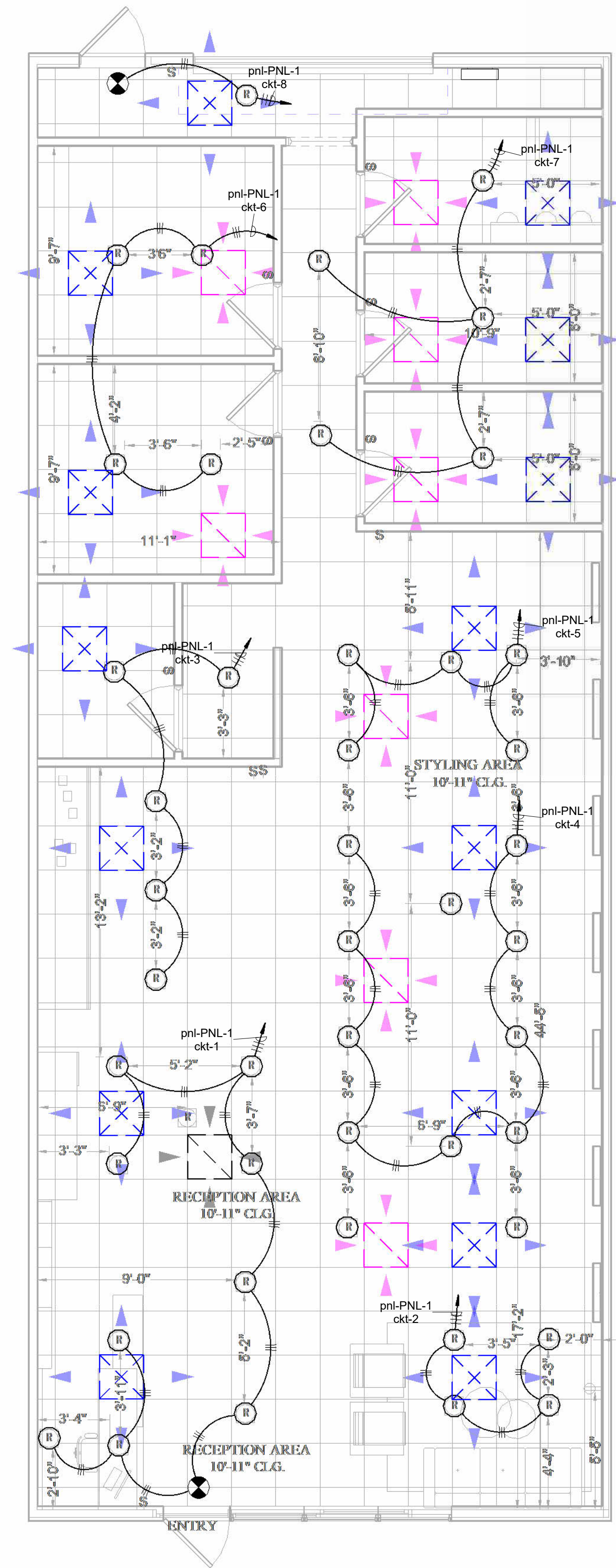
2 LIGHTING PLAN E-1 1/4" = 1'-0"
