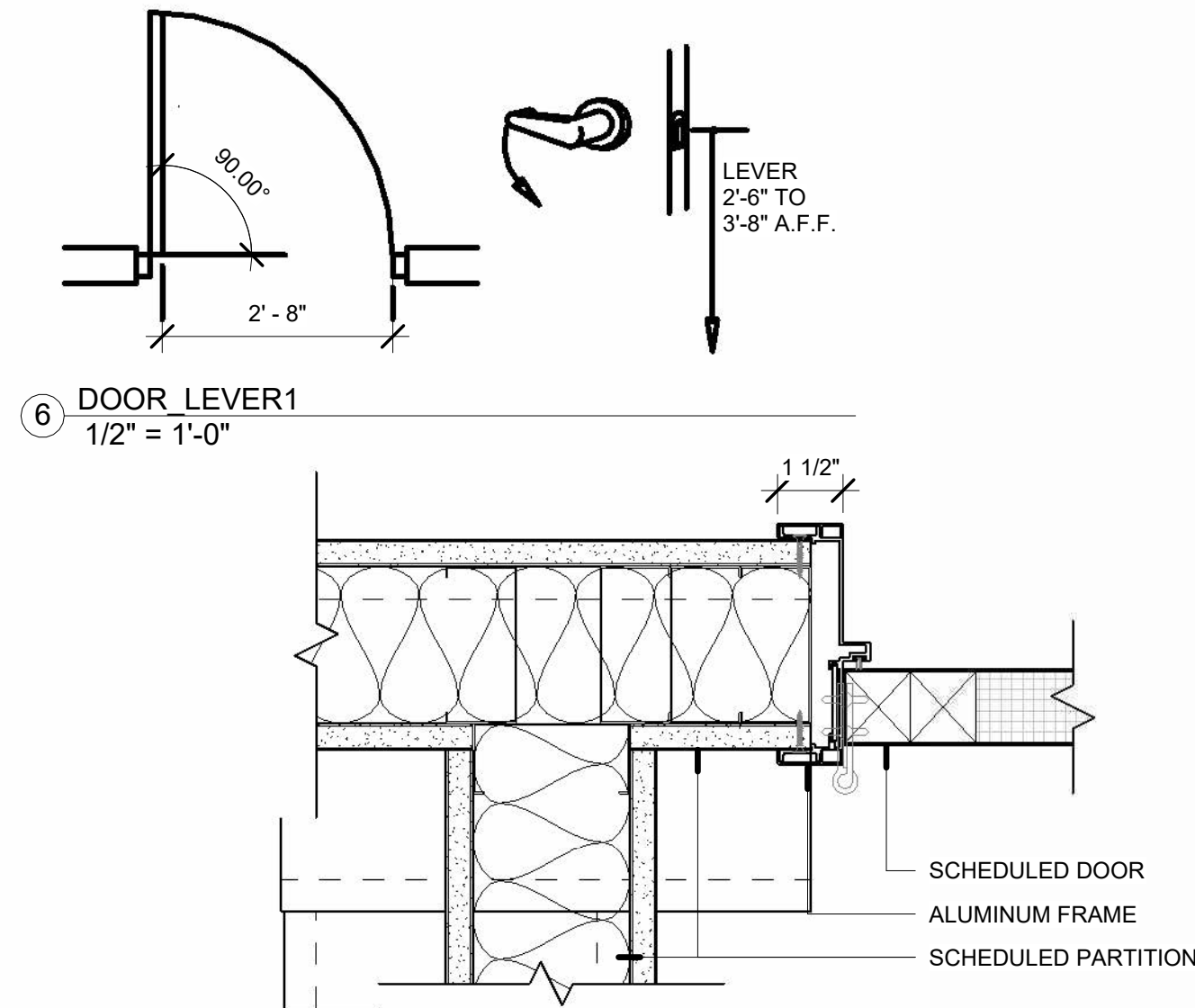
6 DOOR LEVER 1/2" = 1'-0"
