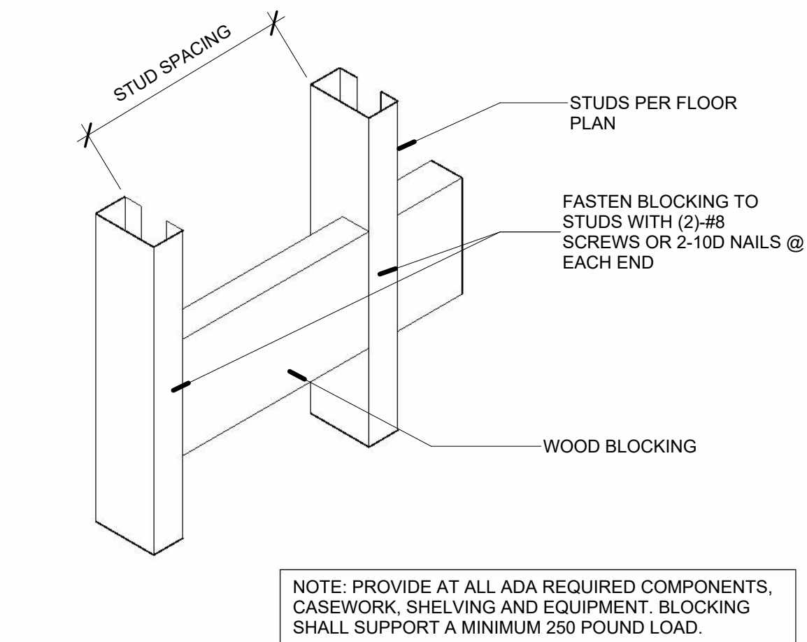
13 Wall Backing Detail 1/4" = 1'-0"
