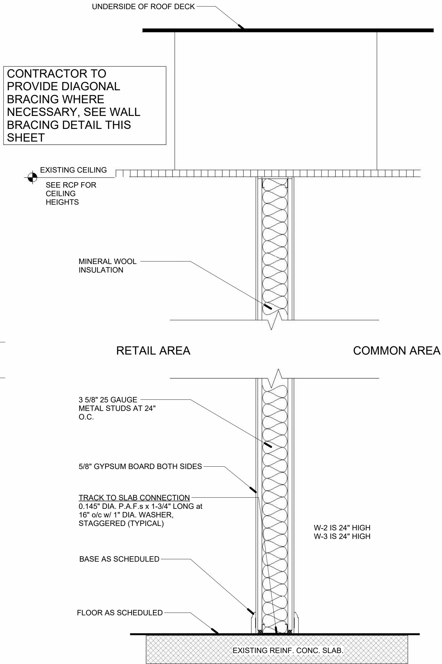
1 TYP INTERIOR WALL TYPE #W3 1 1/2" = 1'-0"
