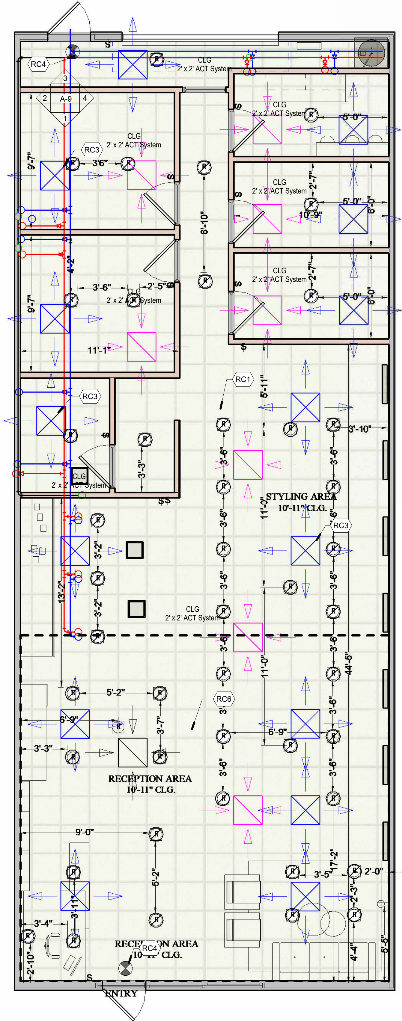
① PROPOSED REFLECTD CEILING PLAN 1/4" = 1'-0"
