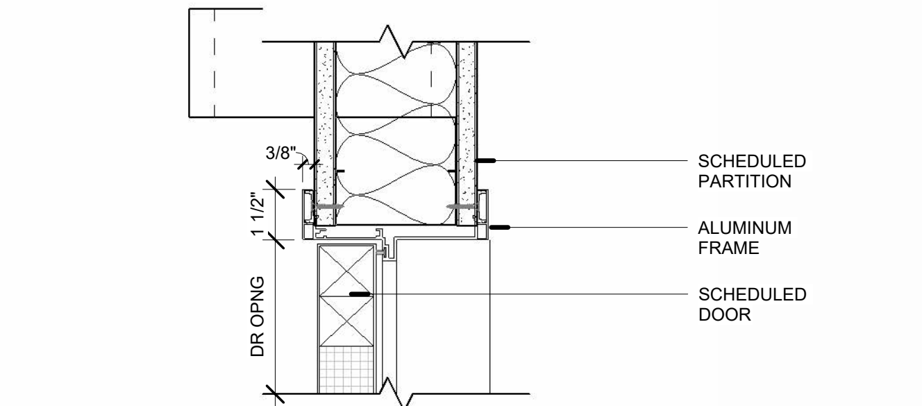
7 HEAD @ STANDARD DOOR 3" = 1'-0"
