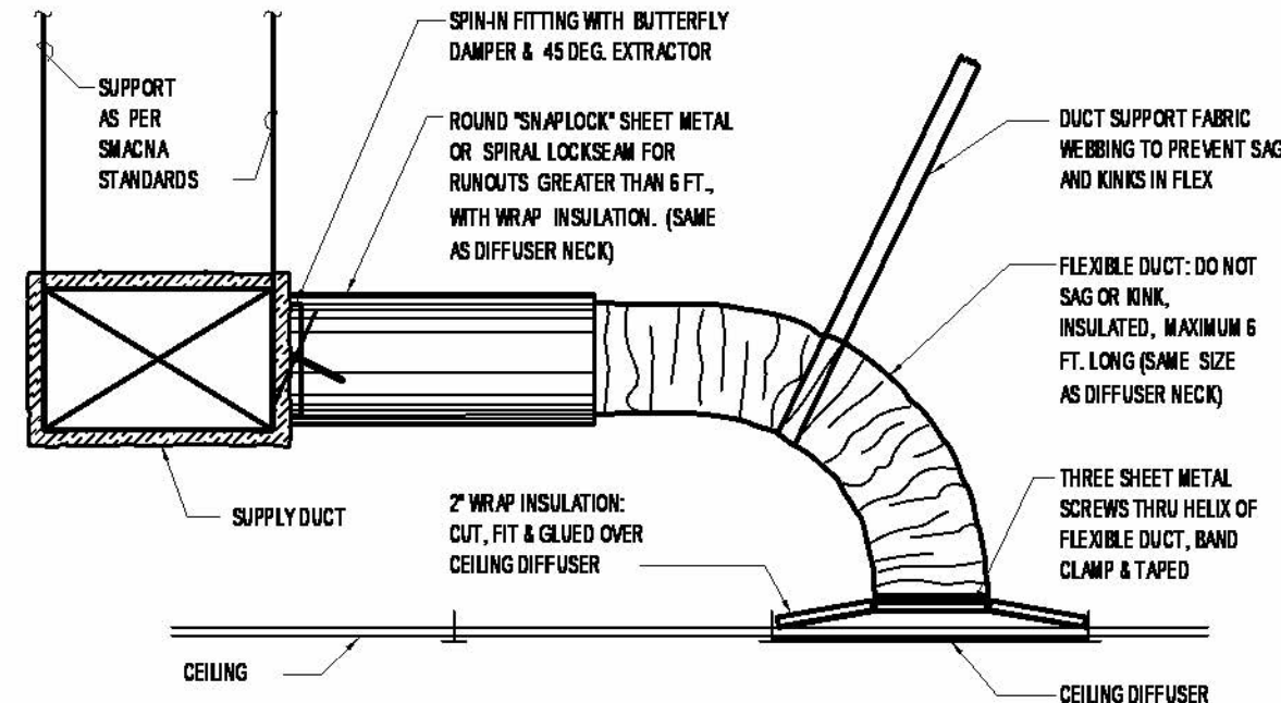
SUPPLY CEILING DIFFUSER RUNOUT DETAIL
