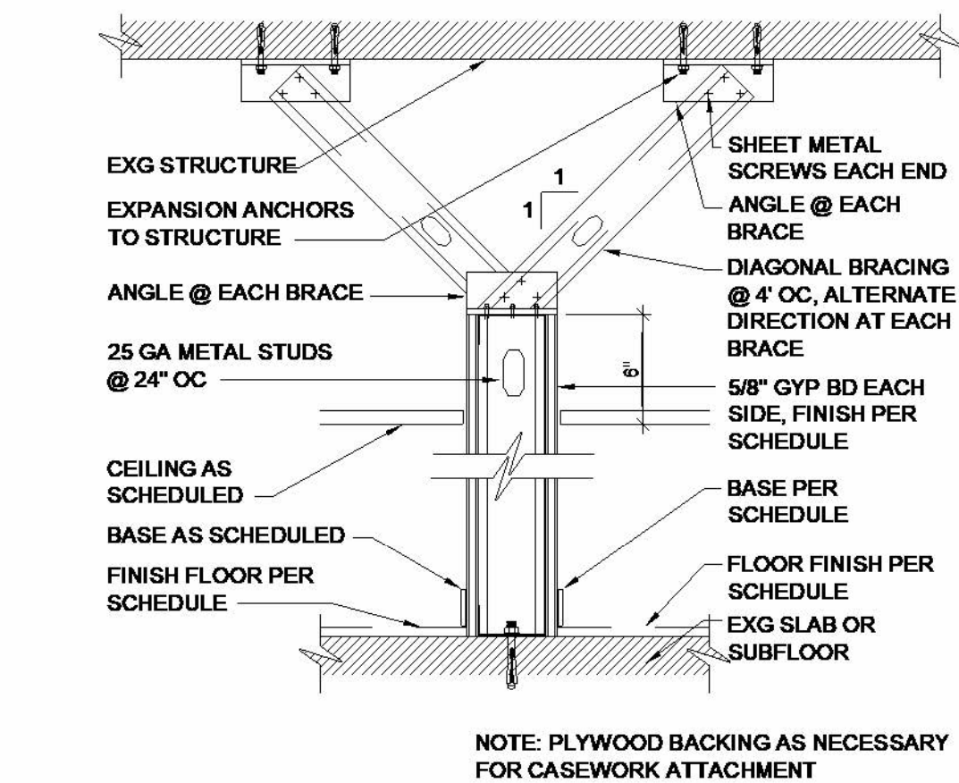
2 WALL BRACING 12" = 1'-0"
