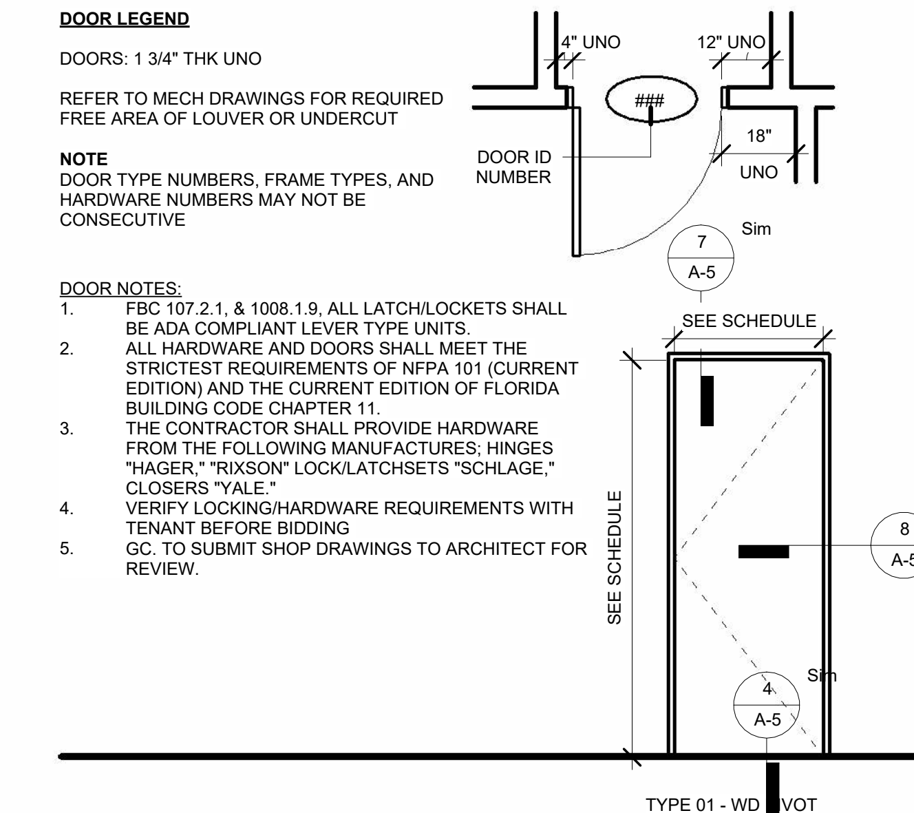
9 DOOR TYPES & LEGEND 3/8" = 1'-0"
