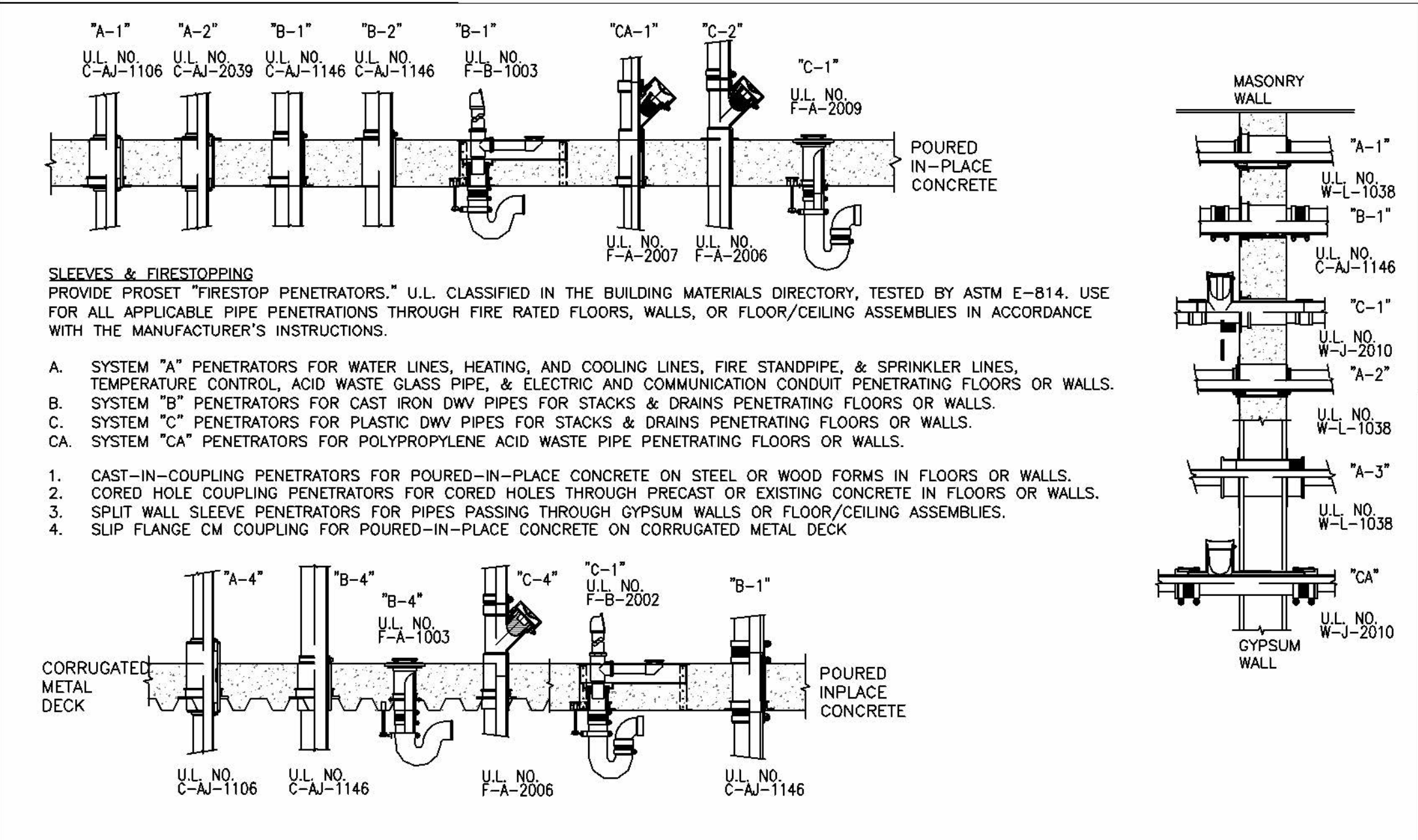
FIRE STOPPING PENETRATION DETAIL
