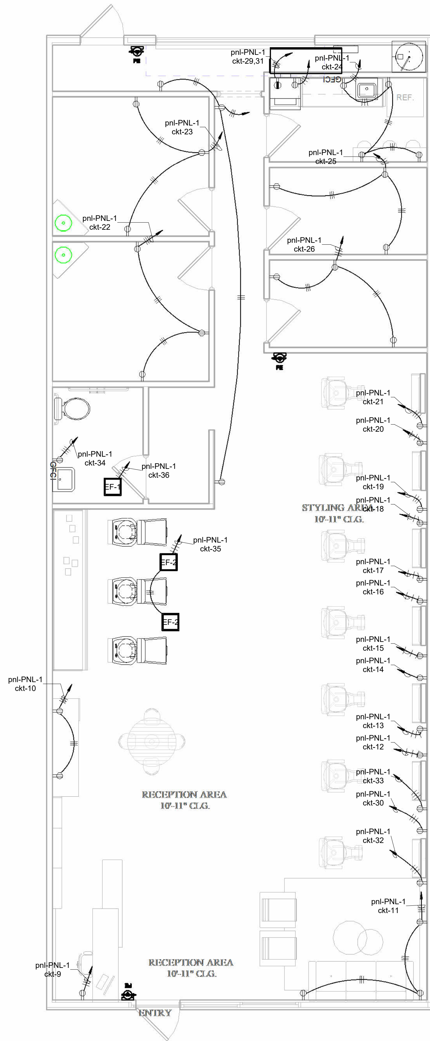
1 POWER FLOOR PLAN E-1 1/4" = 1'-0"
