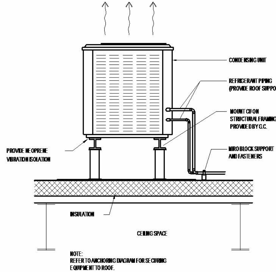
ROOF MOUNTED CU DIAGRAM
