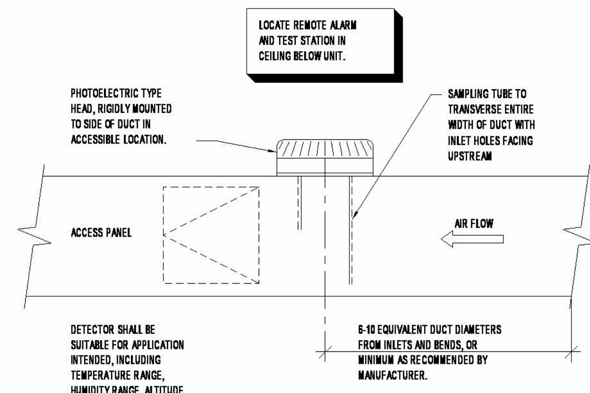
DUCT MOUNTED SMOKE DETECTOR DIAGRAM
