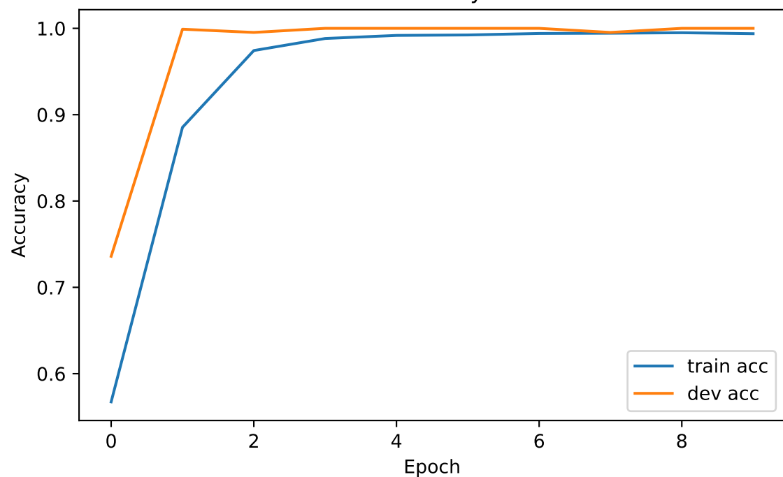
Accuracy
