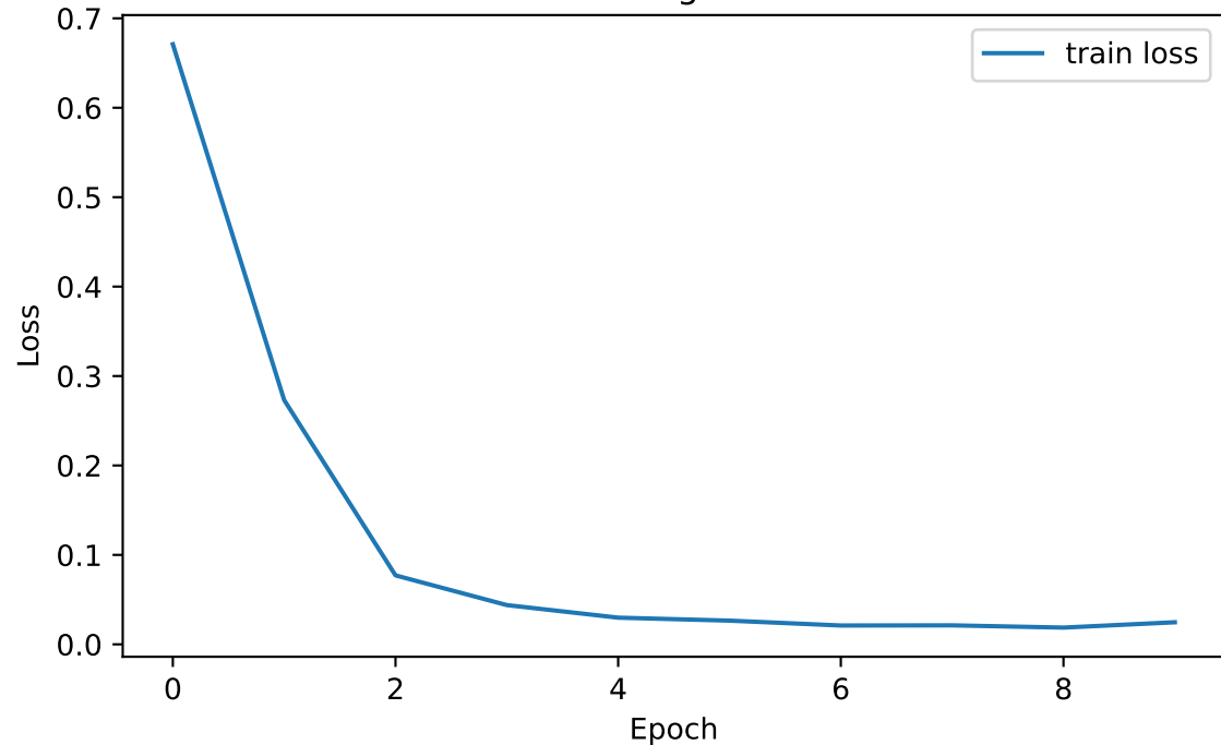
Training Loss
