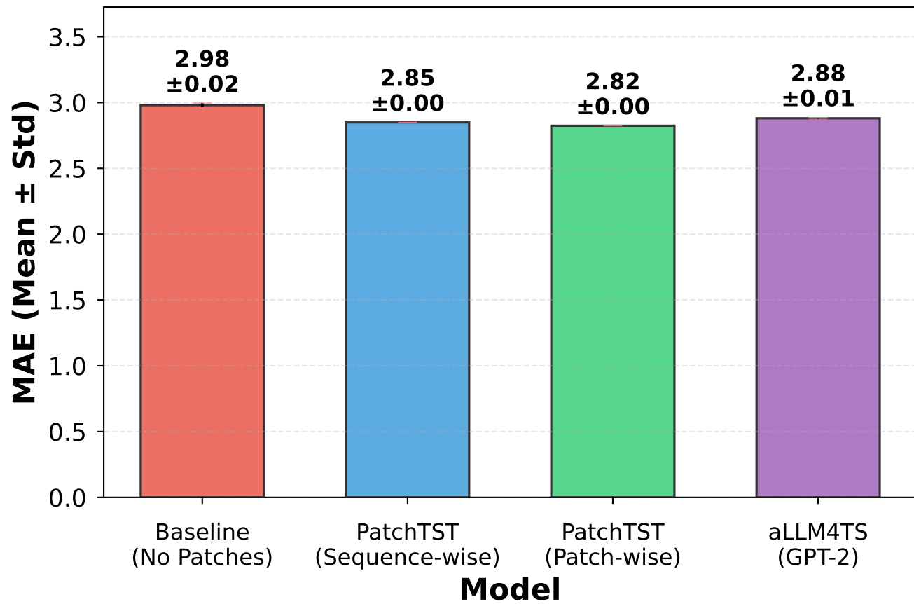
MAE Comparison (Overall)
