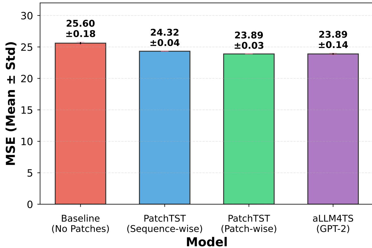
MSE Comparison (Overall)
