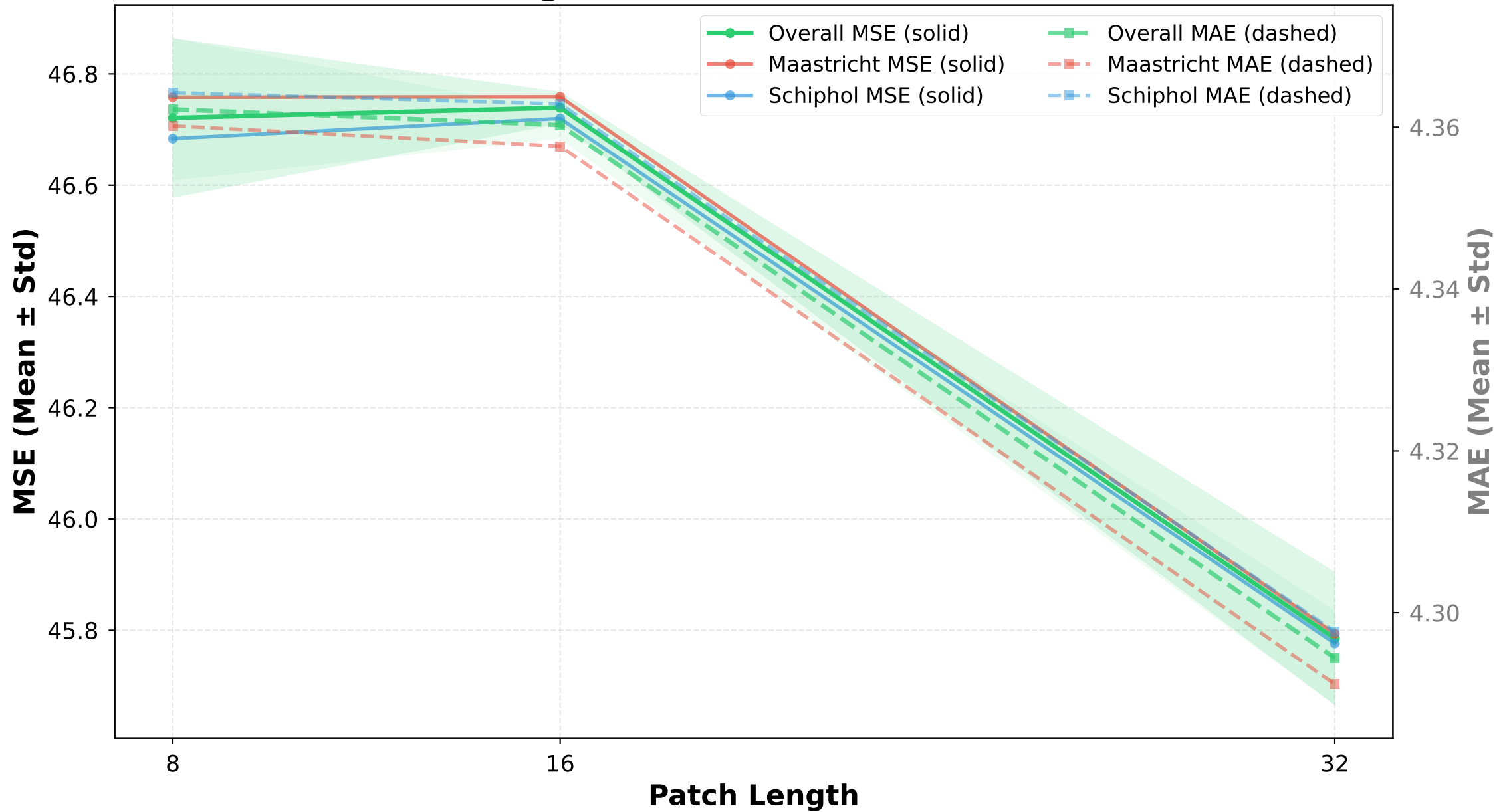
Patch Length Ablation: PatchTST Patchwise
