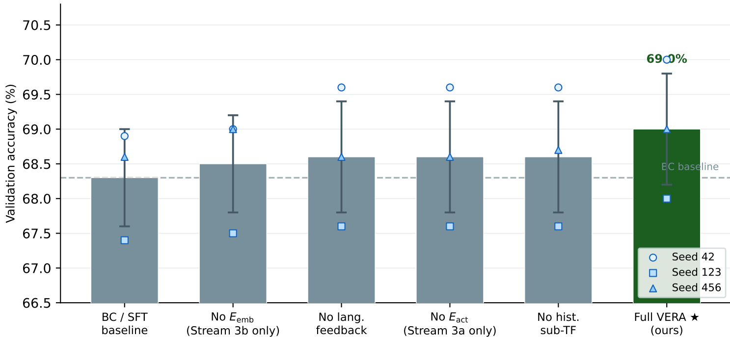
Language-Table ablation — validation action-classification accuracy (3,000 simulated episodes · 90/10 split · 3 seeds each · random baseline = 12.5%)
