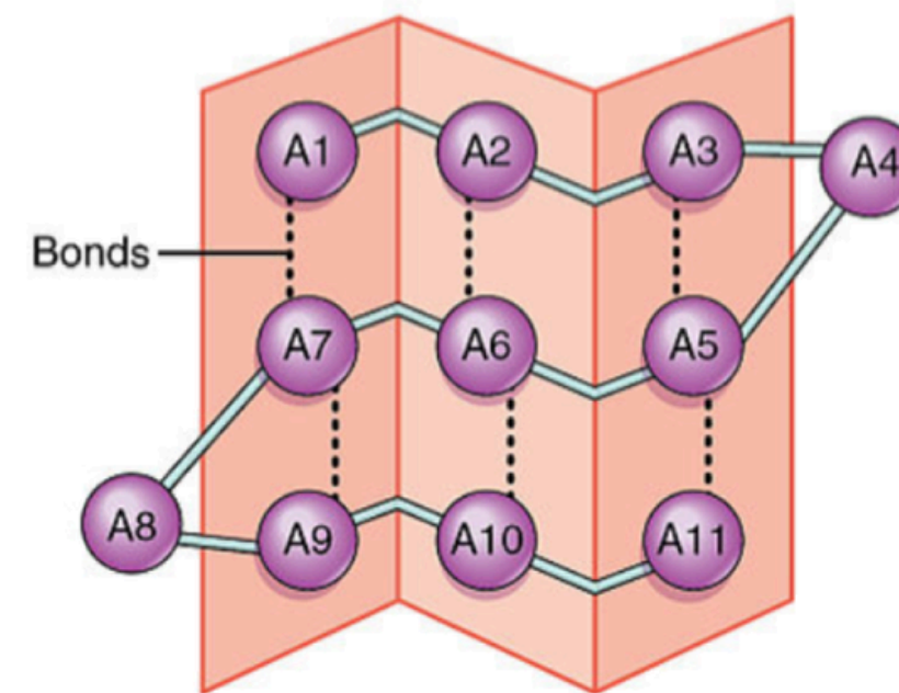
\beta - pleated sheet
