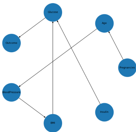
Figure 1: Bayesian Network structure learned using Hill Climbing with AIC score, selected as one of the best-performing models for probabilistic inference and classification.
