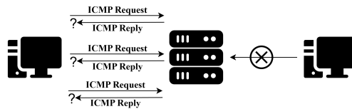
Figura 3.7: ICMP Flood
