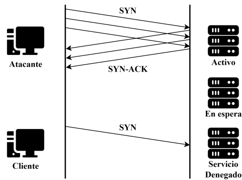
Figura 3.6: SYN Flood
