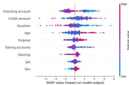
FIGURE 1. SHAP summary plot 2 for German credit dataset.
