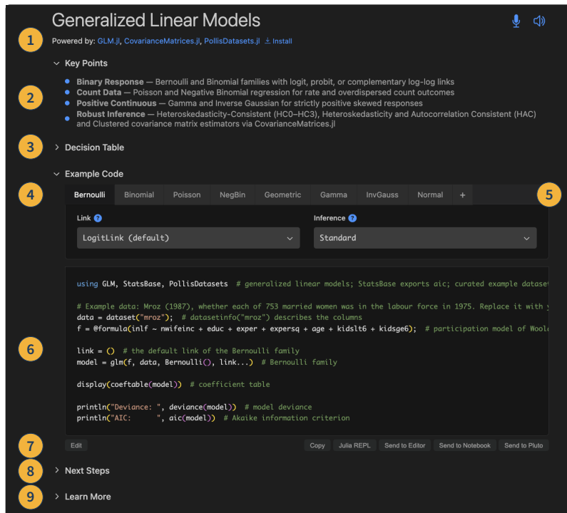
The Generalised Linear Models panel. Choosing a family, a link or a kind of inference (Standard, HC0–HC3, HAC or Clustered) rewrites the example code.
