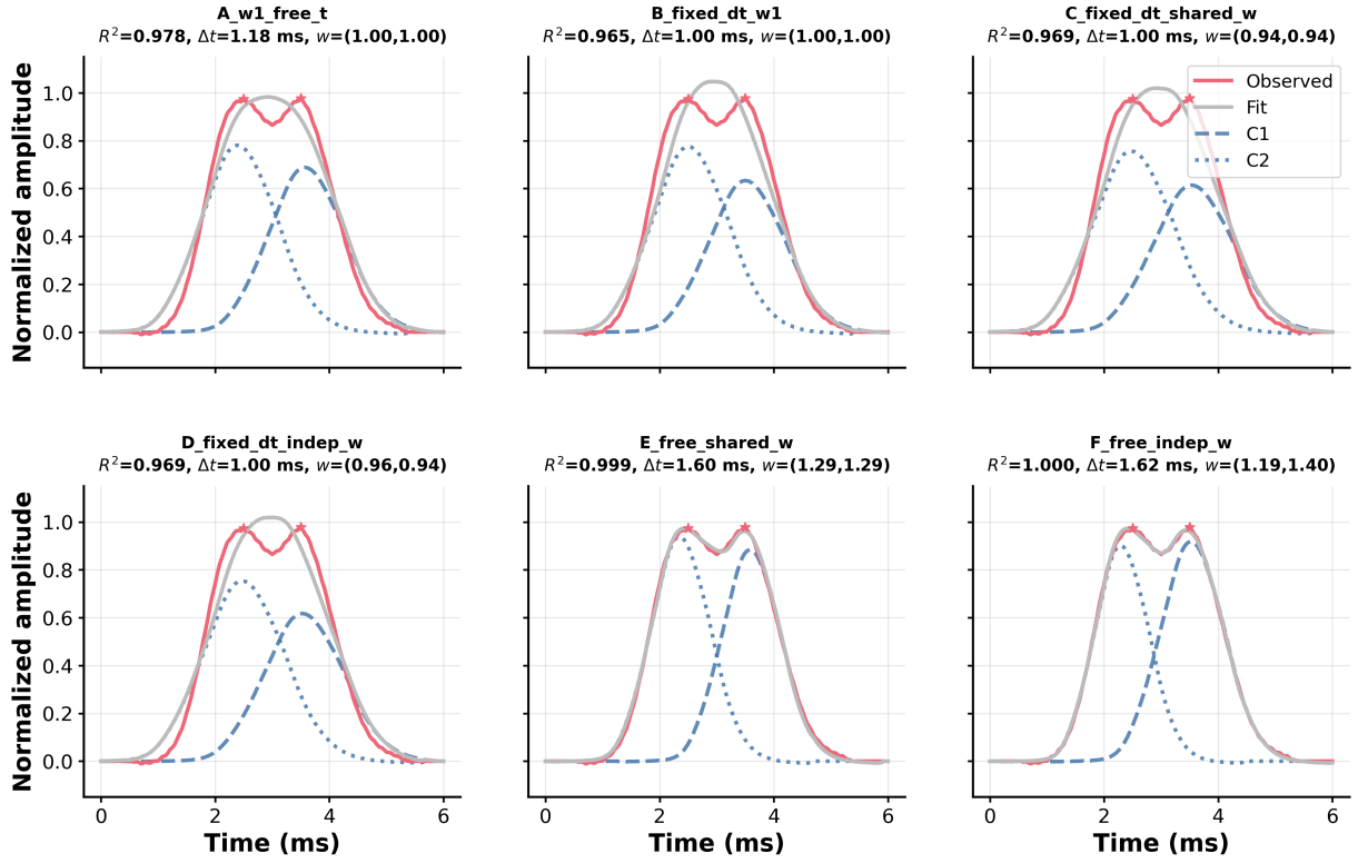
Figure 9: Six ways to model the median double pulse from two median normal components. Varying constraints on \Delta t and the component width scales w produce different fits. Each panel shows the median double (red, stars on the peaks), the model sum of the fitted normals (grey), and the two median normal components C1 and C2 (dashed and dotted blue). From A to F the constraints on \Delta t and w get looser ( w = 1 is the native normal width; w > 1 widens). A already reaches R^2 = 0.978 with native widths. E and F let widths float and push R^2 near 1, with fitted \Delta t drifting away from the observed 1 ms peak spacing and with components broader than the native normal. The characteristic trough of the double pulse shape is recovered only by models E and F.
