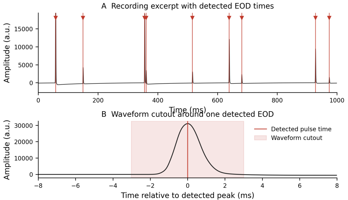
Figure 2: EOD pulse detection on a short Berlin recording excerpt (1s, one electrode channel). Red markers in (A) show eeltracker pulse times. (B) zooms on one detected discharge and shades the short waveform cutout stored for later shape analysis.
