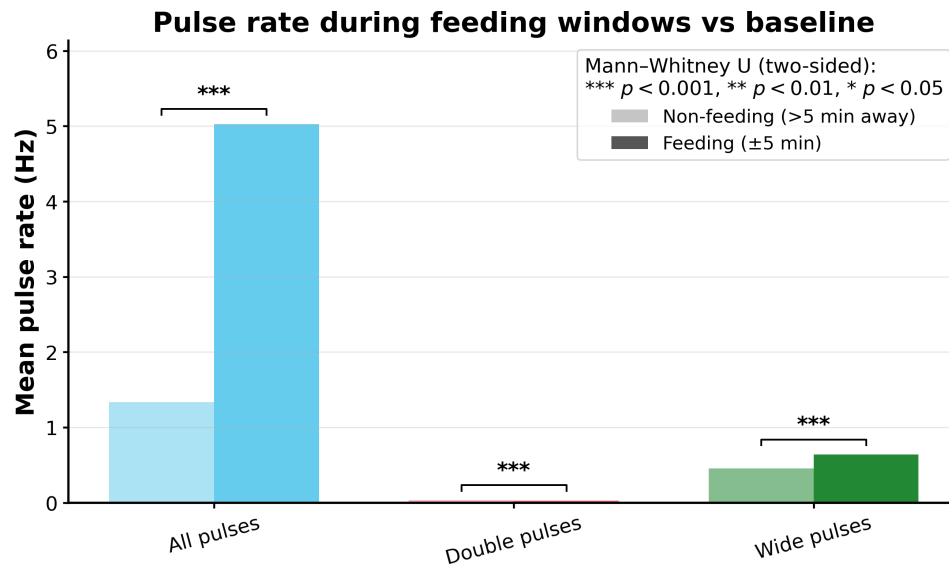
Figure 12: Mean pulse rate in feeding windows ( \pm 5 min) next to the non feeding baseline ( > 5 min away). Blue, red, and green are all, double, and wide pulses. Within each hue the darker bar is feeding and the lighter one is baseline. Brackets mark two-sided Mann–Whitney U tests on minute-level rates (***: p < 0.001 ). Overall activity and wide pulses increase during feeding; doubles stay near the x-axis on this shared mean scale but still differ by the rank test.
