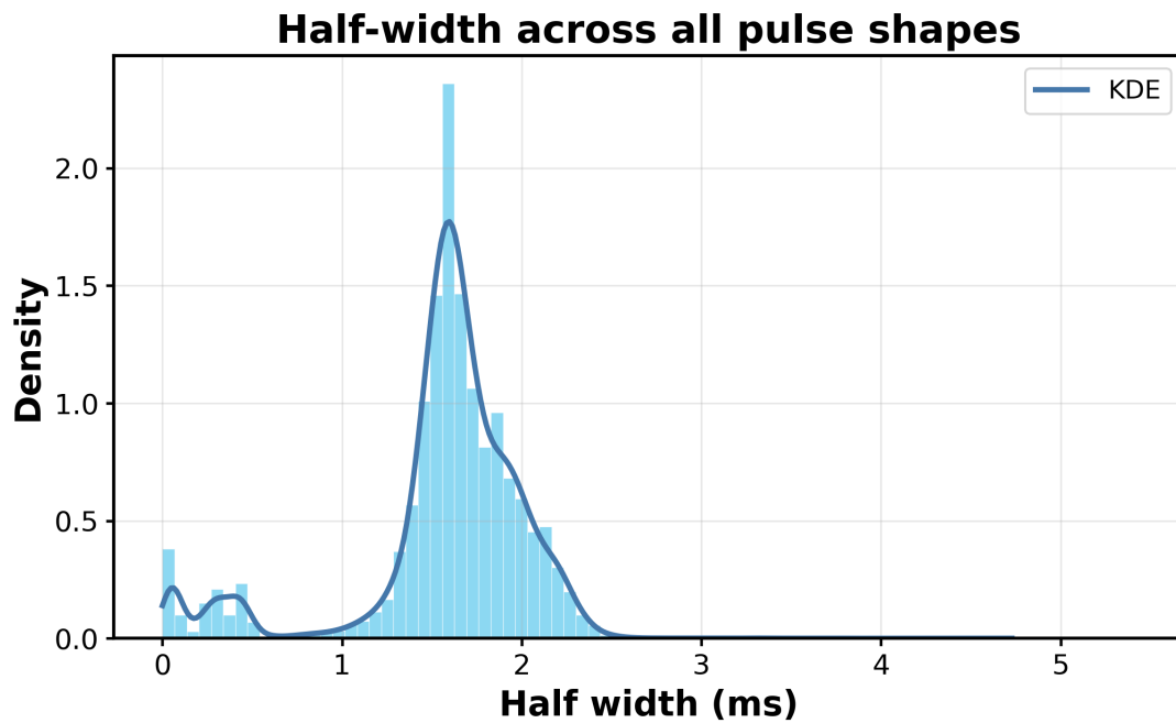
Figure 6: Half-widths of all shapes throcombined in one histogram (light blue bars) with a KDE on top (dark blue). The main mode sits near 1.6 ms with a shoulder toward 2 to 2.5 ms, which is roughly what mixing the three classes above would produce.
