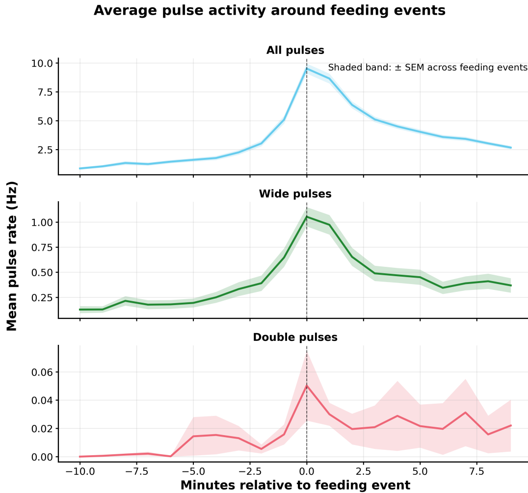
Figure 13: Minute by minute rate around feeding, one panel each for all pulses, wide pulses, and double pulses, each with its own y-axis. Coloured traces are means across matched feeding events (blue - all pulses, green - wide, red - double). The matching washed out band is \pm SEM over those events ( scipy.stats.sem in correlate_activity_with_feeding.py ). The dashed vertical line is the logged feeding time that each trace was aligned to. Overall rate starts climbing about two minutes early, hits roughly 9 Hz at time zero, then decays until the end of the time window at +10 minutes. Wides follow the same shape at lower amplitude (peak near 1.1 Hz). On the double-pulse panel a short peak near 0.05 Hz appears at time zero.
