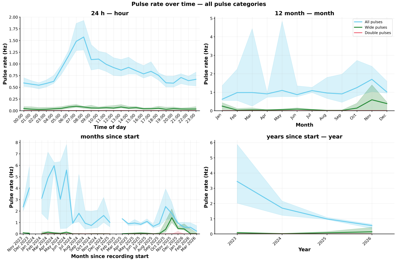
Figure 10: Pulse rate across different timescales (24 h, monthly, yearly), with all pulses, wide pulses, and double pulses in the same panels. Thick traces are active session medians (light blue all pulses, pink doubles, dark green wides). The washed out bands show bootstrap 95% CIs. Top Left: 24 h scale with hourly bins. Top Right: Calendar months with monthly bins. Bottom Left: Chronological monthly record with monthly bins. Bottom Right: Yearly bins from recording start in 2023 to end in 2026.
