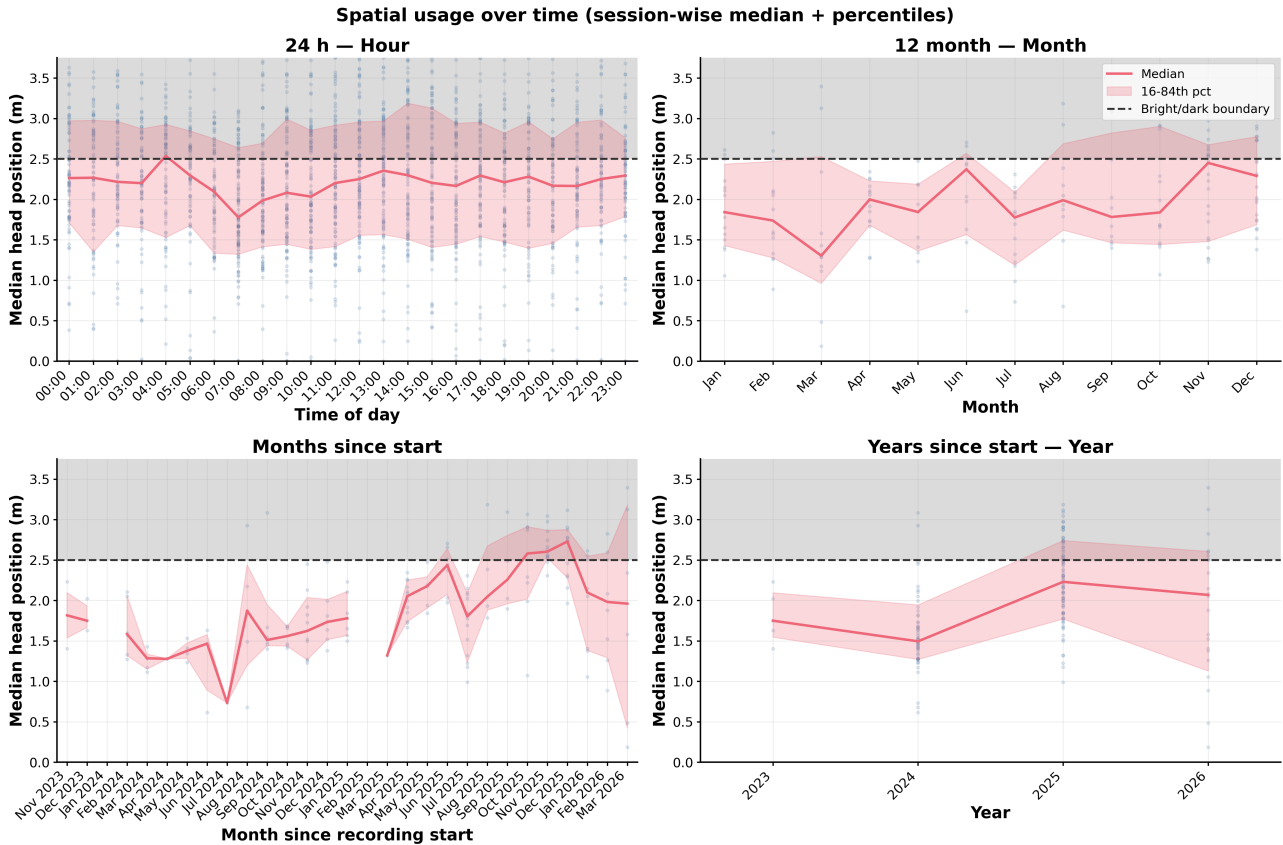
Figure 15: Head position through the same four timescales as the activity figure. The pink line is the session wise median, the light pink band the 16th to 84th percentile, and the faint blue dots the session values themselves. Everything above the dashed line (grey wash) is the dark half of the tank past 2.5 m. Medians usually sit on the bright side, slide toward the front mid morning, and wander over months, including a late 2025 stretch nearer the dark boundary.
