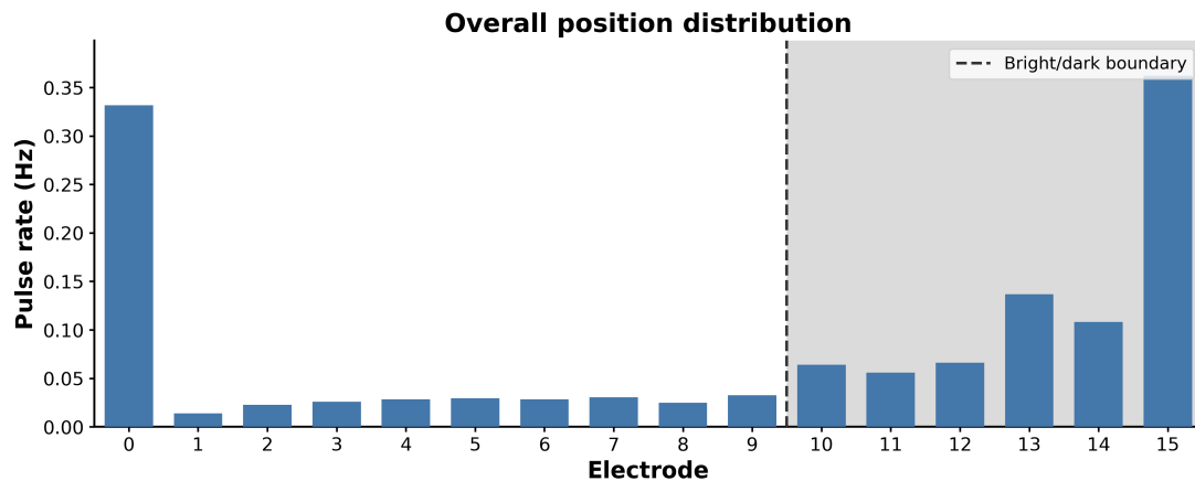
Figure 14: Where along the 16 electrode line the pulses land when hourly bins are collapsed. Blue bars give pulse rate per electrode. The dashed vertical line is the bright/dark cut at 2.5 m, and the light grey wash marks the dark half (electrodes 10 to 15). Animals spend most time at the two ends (0 and 15), and the dark mid electrodes stay busier than the bright mid stretch.
