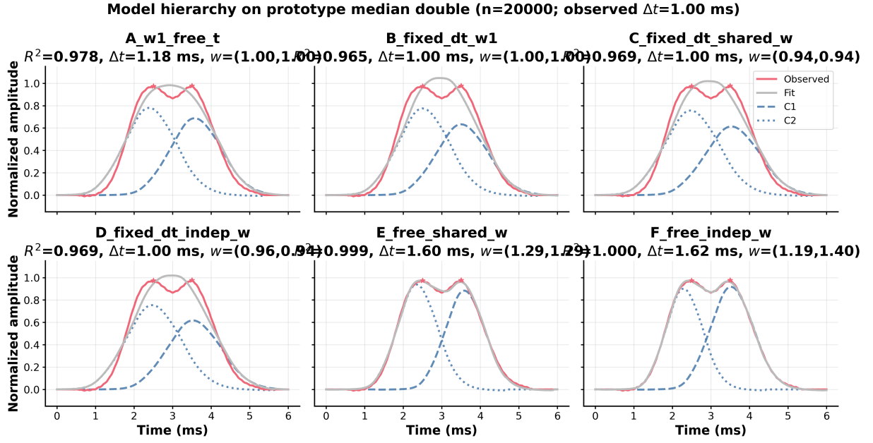
Figure 9: Six ways to model the median double pulse from two median normal components. Varying constraints on \Delta t and the component widths w produce different fits. Each panel shows the median double (red, stars on the peaks), the model sum of the fitted normals (grey), and the two median normal components C1 and C2 (dashed and dotted blue). From A to F the constraints on \Delta t and the component widths w get looser. A already reaches R^2 = 0.978 with native widths. E and F let widths float and push R^2 near 1, with fitted \Delta t drifting away from the observed 1 ms peak spacing. The characteristic trough of the double pulse shape is recovered only by models E and F.
