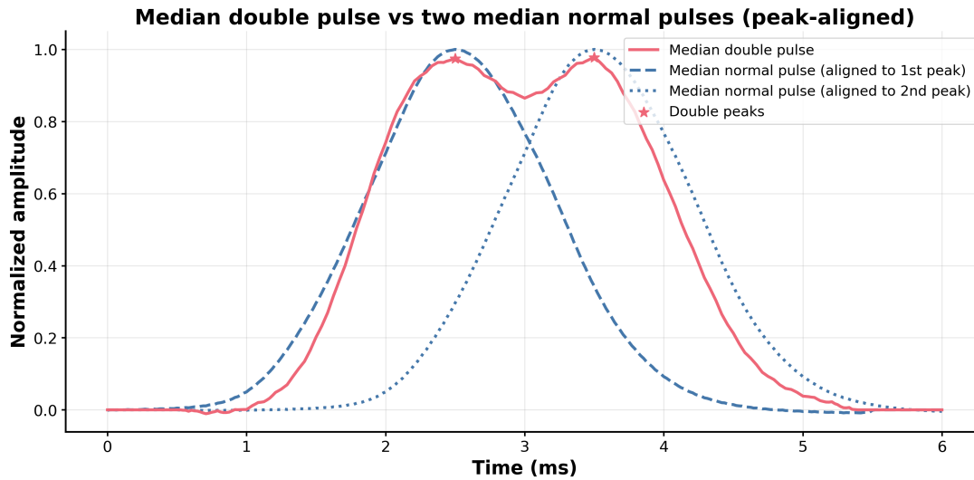
Figure 8: Two median normal pulses aligned to the peaks of the median double pulse. The solid pink trace is the median double, with red stars on its peaks. The dashed and dotted blue curves are the median normal, shifted along the x-axis so each sits under one of those peaks. The trough lands where the two normals cross, which is what you would expect if the double were just a short \sim 1 ms doublet of the normal shape.
