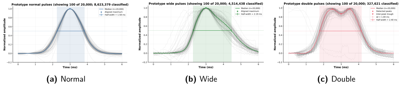
Figure 4: Median waveforms for the three classes. The thick coloured trace is the class median ( n = 20,000 ). The thin grey pulses are 100 example pulses per class. The stars mark where the waveforms were aligned (peak for normal and wide, trough between peaks for double). Normals are short and single peaked, wides stretch out with a slower falling edge, and doubles carry two peaks about 1 ms apart.
