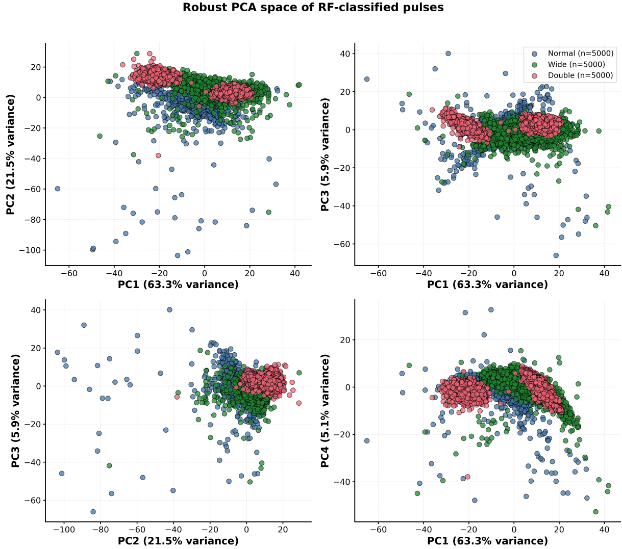
Figure 7: RF labelled pulses in Robust PCA space, 5000 examples per class. Blue points represent normal pulses, green wide pulses, and red double pulses. The four panels are different PC pairings. Doubles form two distinct clouds; normals show higher variability, especially along PC2. Wides are located between double and normal regions while leaning more into the double pulse cluster. In the PC3/PC4 vs. PC1 views the doubles look like two clumps rather than one.
