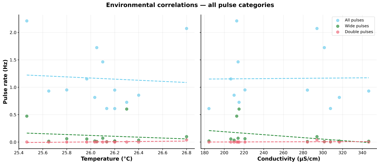
Figure 11: Environmental correlations of pulse rate in Hz with tank temperature in ^{\circ}\text{C} (left) and conductivity in \mu\text{S cm}^{-1} (right). Each cloud is a pulse category (light blue - all pulses, red - double, green - wide), with a dashed line of the same colour indicating the linear fit ( n = 13 months). The only significant Pearson correlation is double vs temperature ( p = 0.023 ). In a Spearman rank correlation all three traces are not significant. Special-shape rates sit well below the all-pulse scatter.
