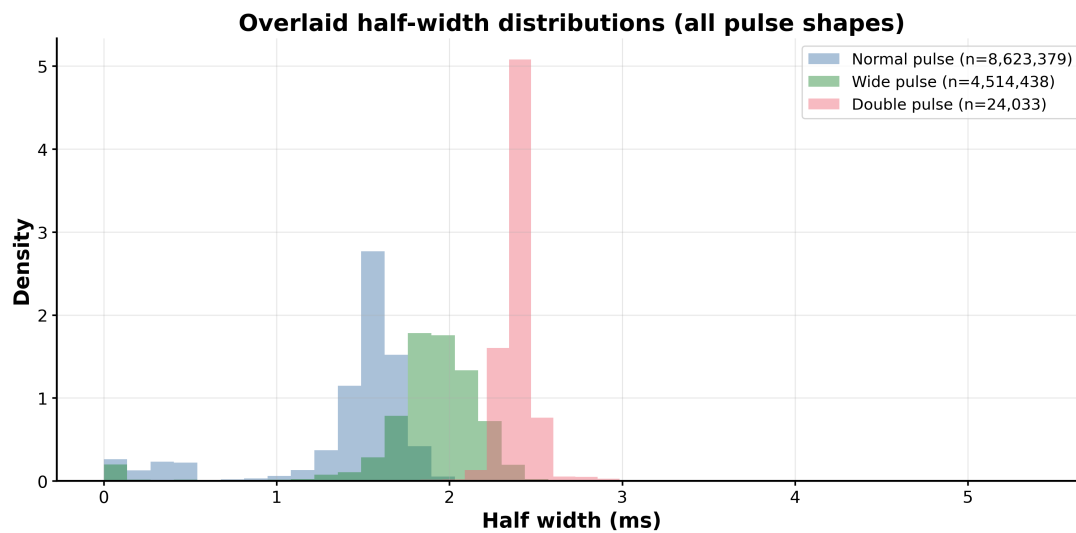
Figure 5: Half width densities for the three classes drawn on top of each other, with normal shown in blue, double in pink, and wide pulses in green. Normal and wide share a lot of support around 1.5 to 2 ms, while doubles pile up in a narrow ridge near 2.4 ms.
