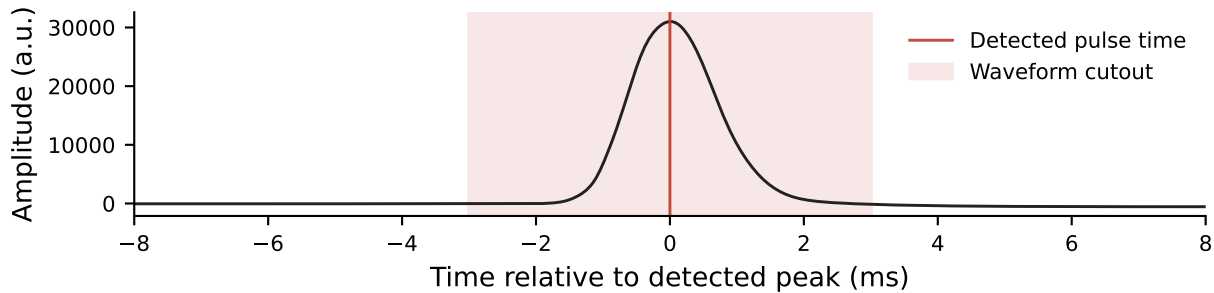
B Waveform cutout around one detected EOD
