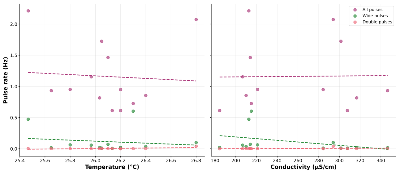
Figure 10: Environmental correlations of pulse rate with tank temperature (left) and conductivity (right). Each cloud is a pulse category with a dashed linear fit ( n = 13 months). The only significant Pearson correlation is double vs temperature ( p = 0.023 ). In a Spearman rank correlation all three traces are not significant. Special-shape rates sit well below the all-pulse scatter.
