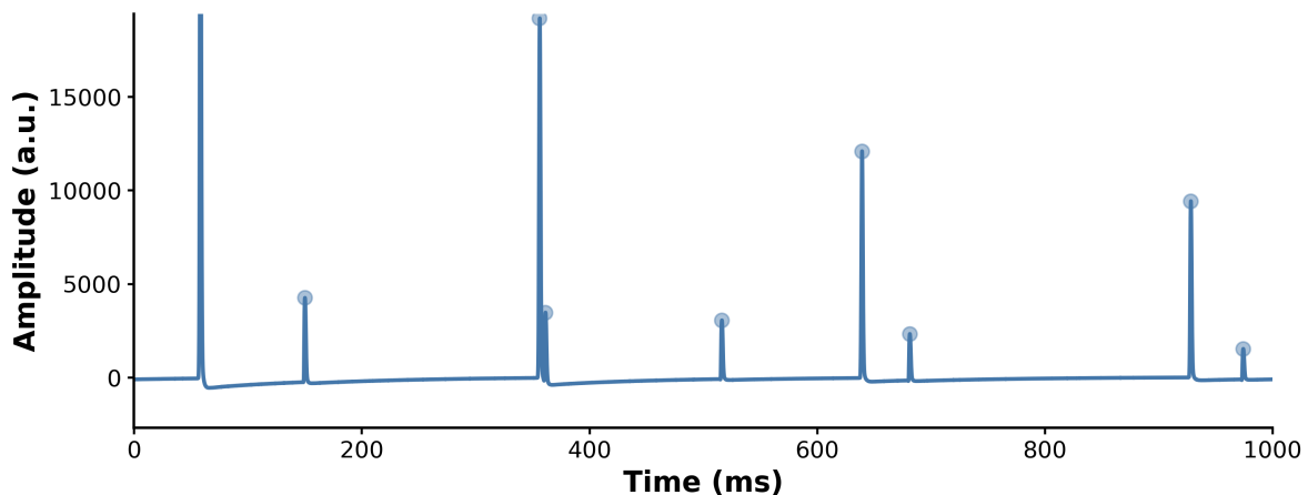
Figure 2: One-second excerpt from a Berlin tank recording (single electrode channel). Low- and high-amplitude discharges appear in the same window. Both enter the downstream counts and shape classes; there is no amplitude or volley filter.
