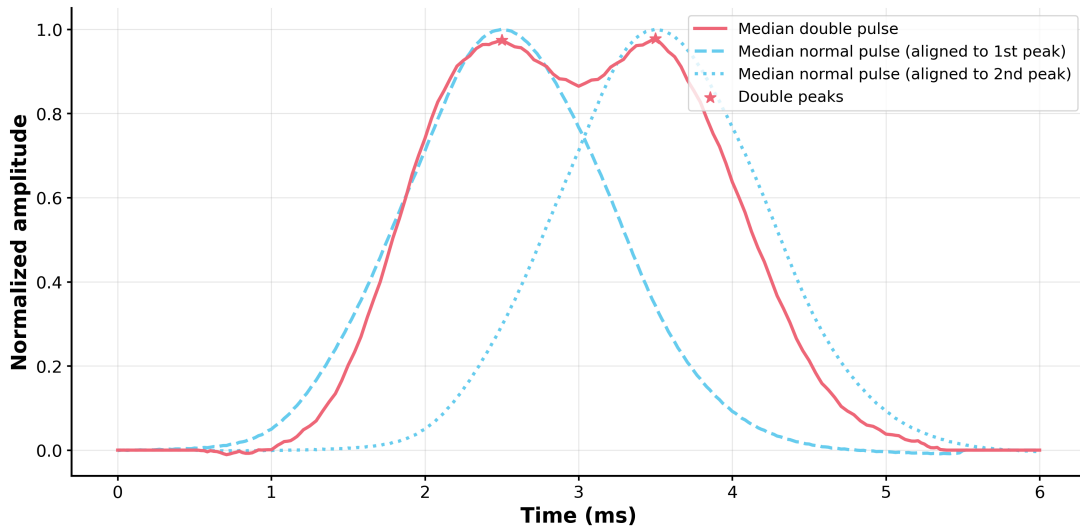
Figure 7: Two median normal pulses aligned to the peaks of the median double pulse. The trough lands where the two normals cross. A pure short doublet of unmodified normals already looks similar, but the quantitative fits (Figure 8) show that matching the trough requires broader components.
