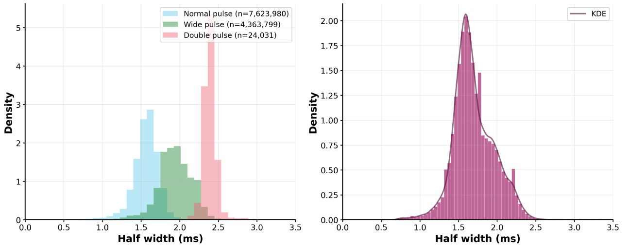
Figure 5: Half-width distributions for the three waveform classes. Left: class-wise densities; legend n counts pulses with measurable half width \geq 0.7 ms (not the full RF class totals). Right: all classes pooled, with a KDE overlay. Pulses shorter than 0.7 ms are excluded to suppress noise / misclassification artefacts. Normal and wide share support around 1.5 to 2 ms, while doubles form a narrow ridge near 2.4 ms. The pooled mode sits near 1.6 ms with a shoulder toward 2 to 2.5 ms.
