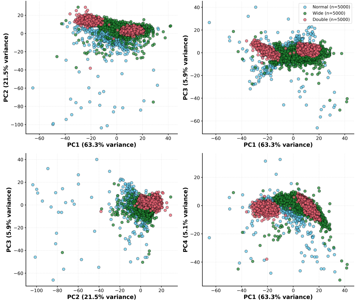
Figure 6: RF labelled pulses in PCA space (5000 examples per class; panels show different PC pairings). Doubles form two dense clouds; normals show higher variability, especially along PC2. Wides lie between normal and double regions and partially overlap the double cloud.
