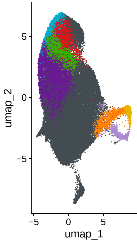
shc_clusters
