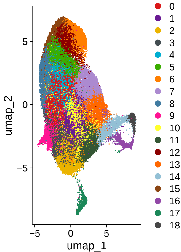
res1.2_clusters
