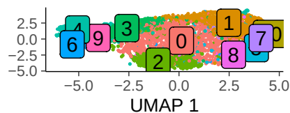
Progenitor clusters (RPCA)
