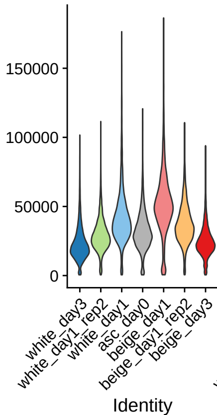
nCount_RNA
