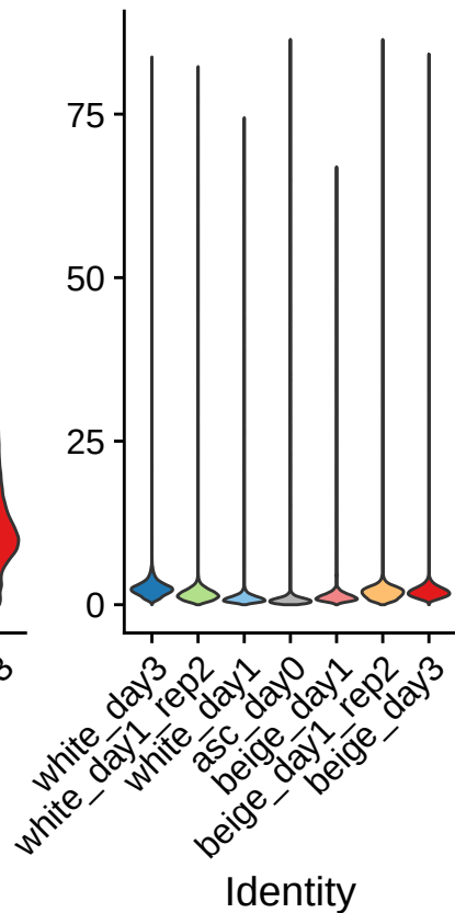
percent.mt
