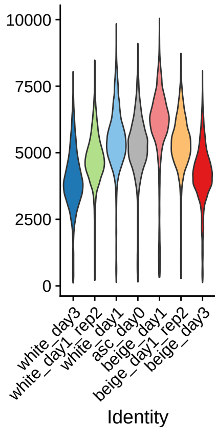
nFeature_RNA
