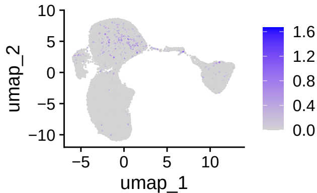
CARMIL2
