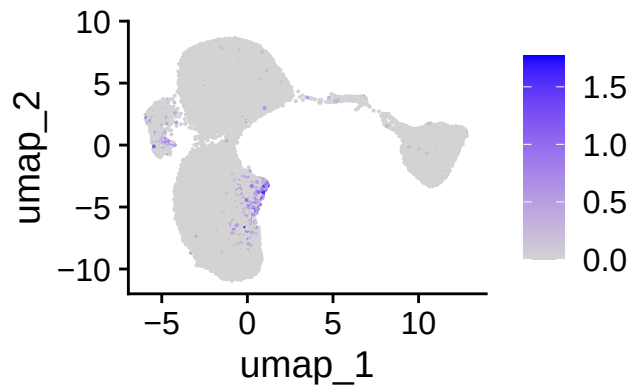
DERL3
