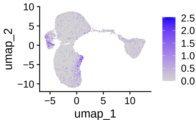
SEC11C
