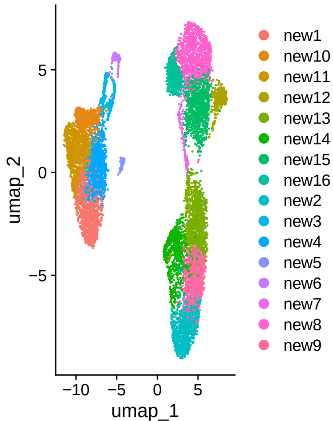
shc_clusters
