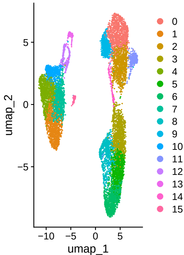
res0.8_clusters
