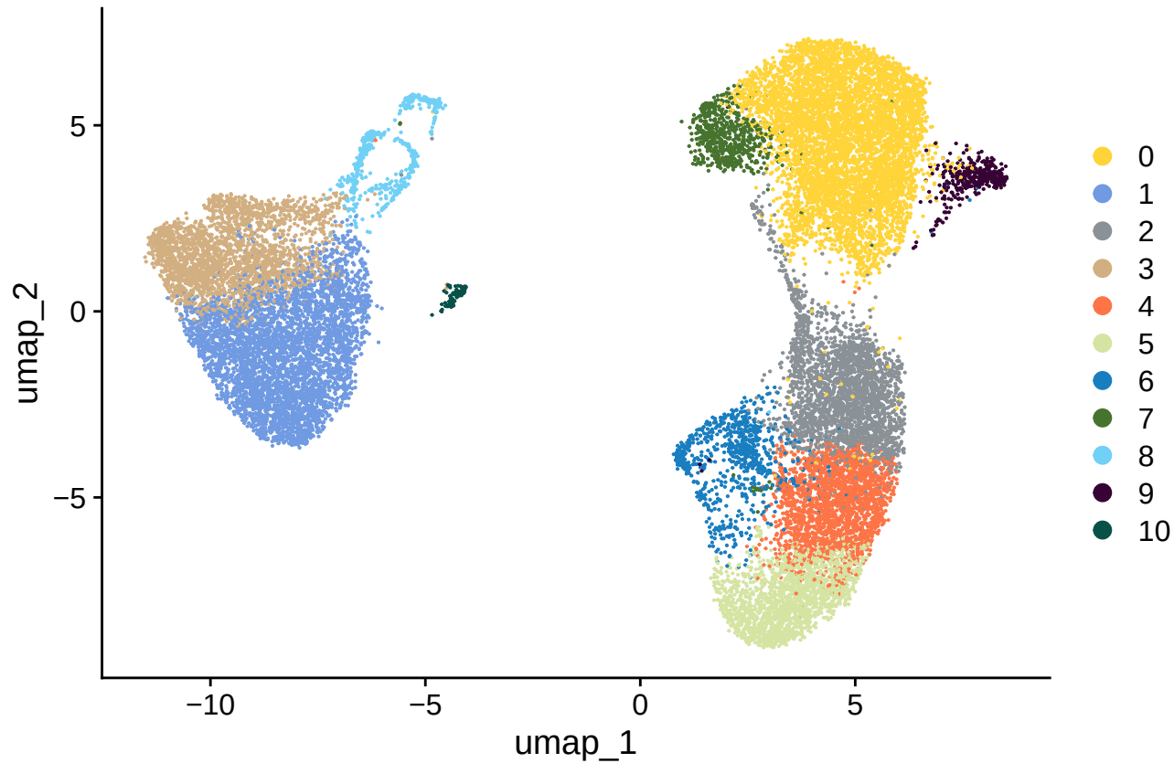
res0.6_clusters
