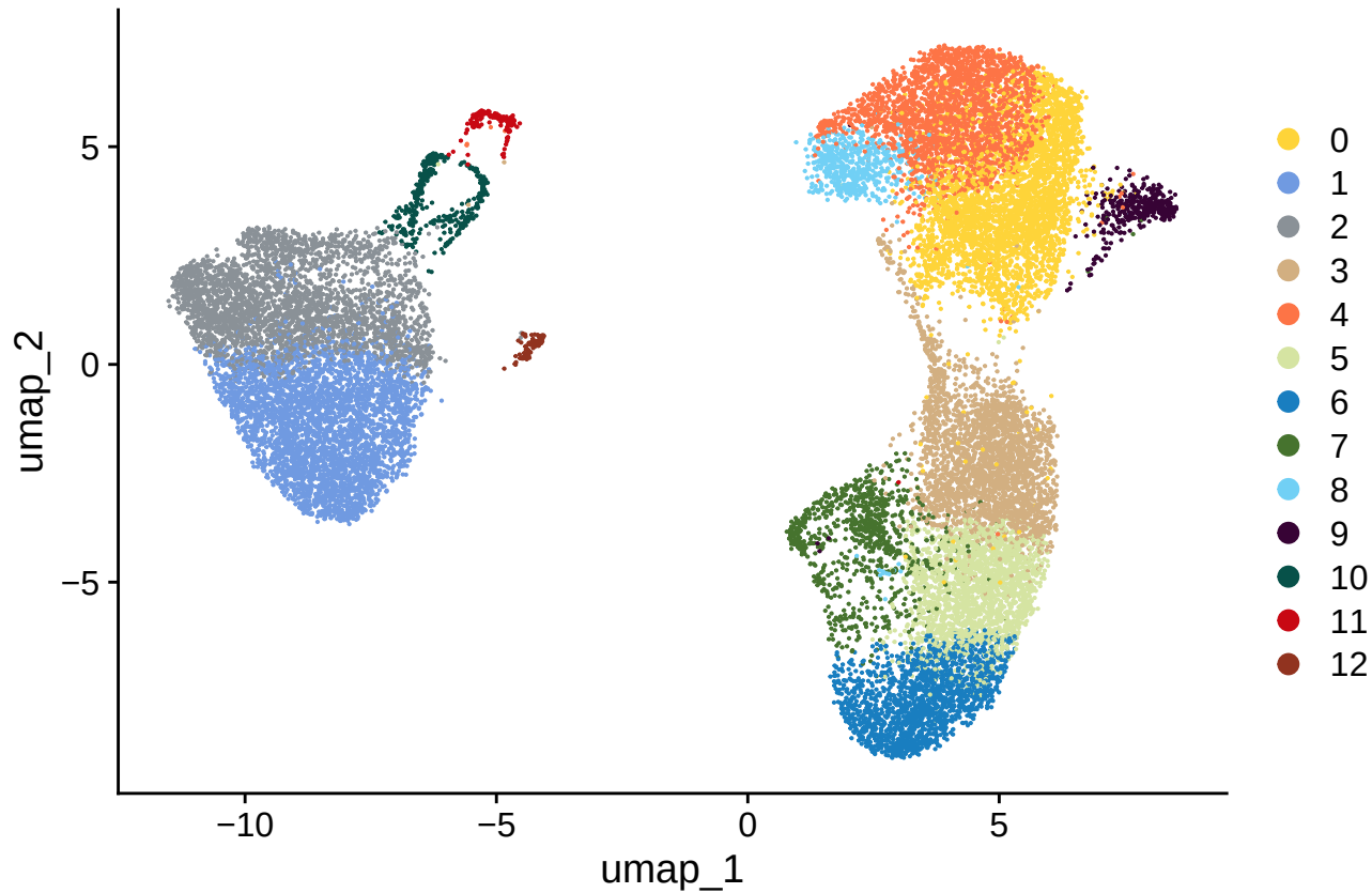
res0.7_clusters
