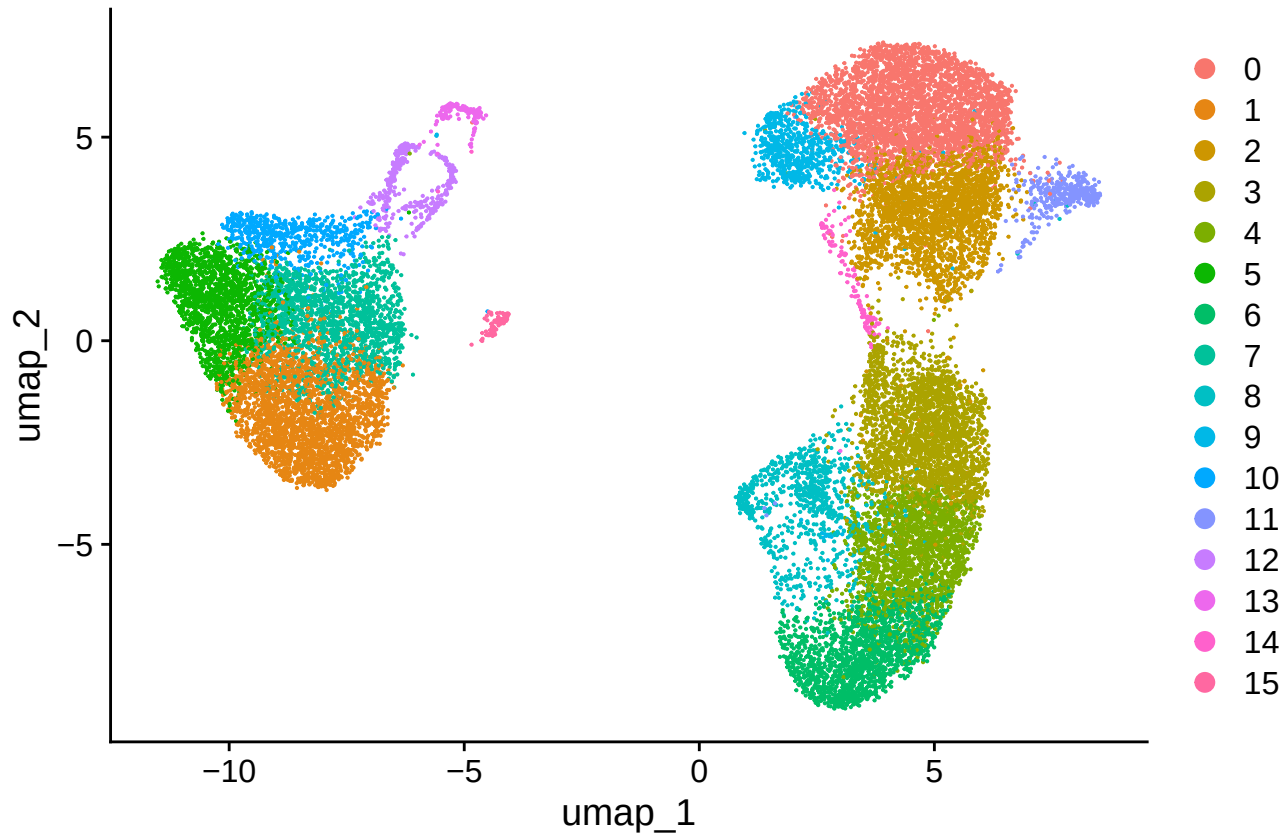
res1_clusters
