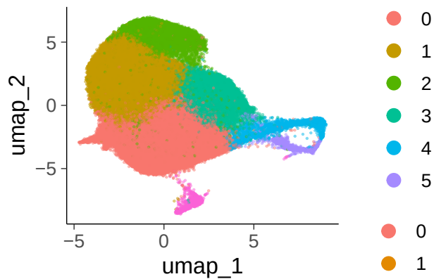
res0.8_clusters
