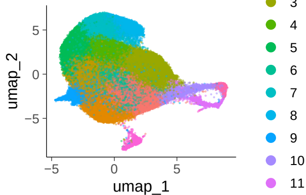
res0.8_clusters
