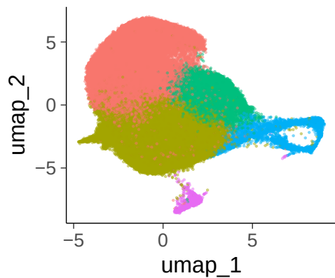
res0.5_clusters
