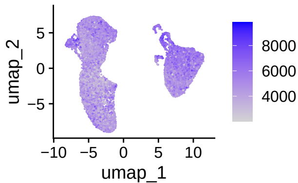
nFeature_RNA
