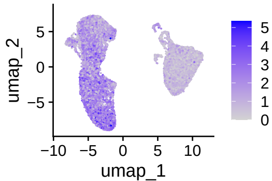
nFeature_RNA
