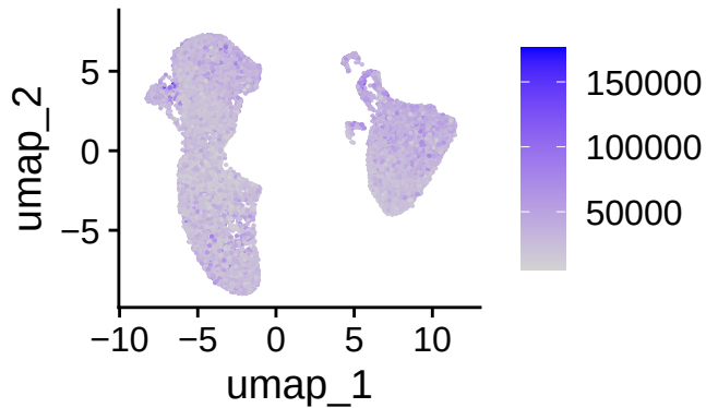
nCount_RNA
