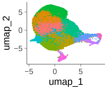
res0.5_clusters
