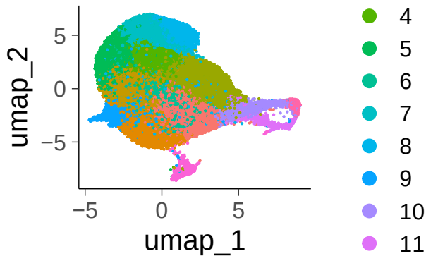
res0.8_clusters
