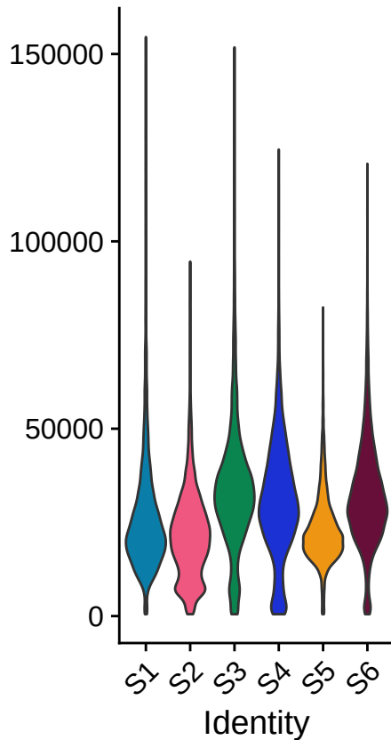
nCount_RNA
