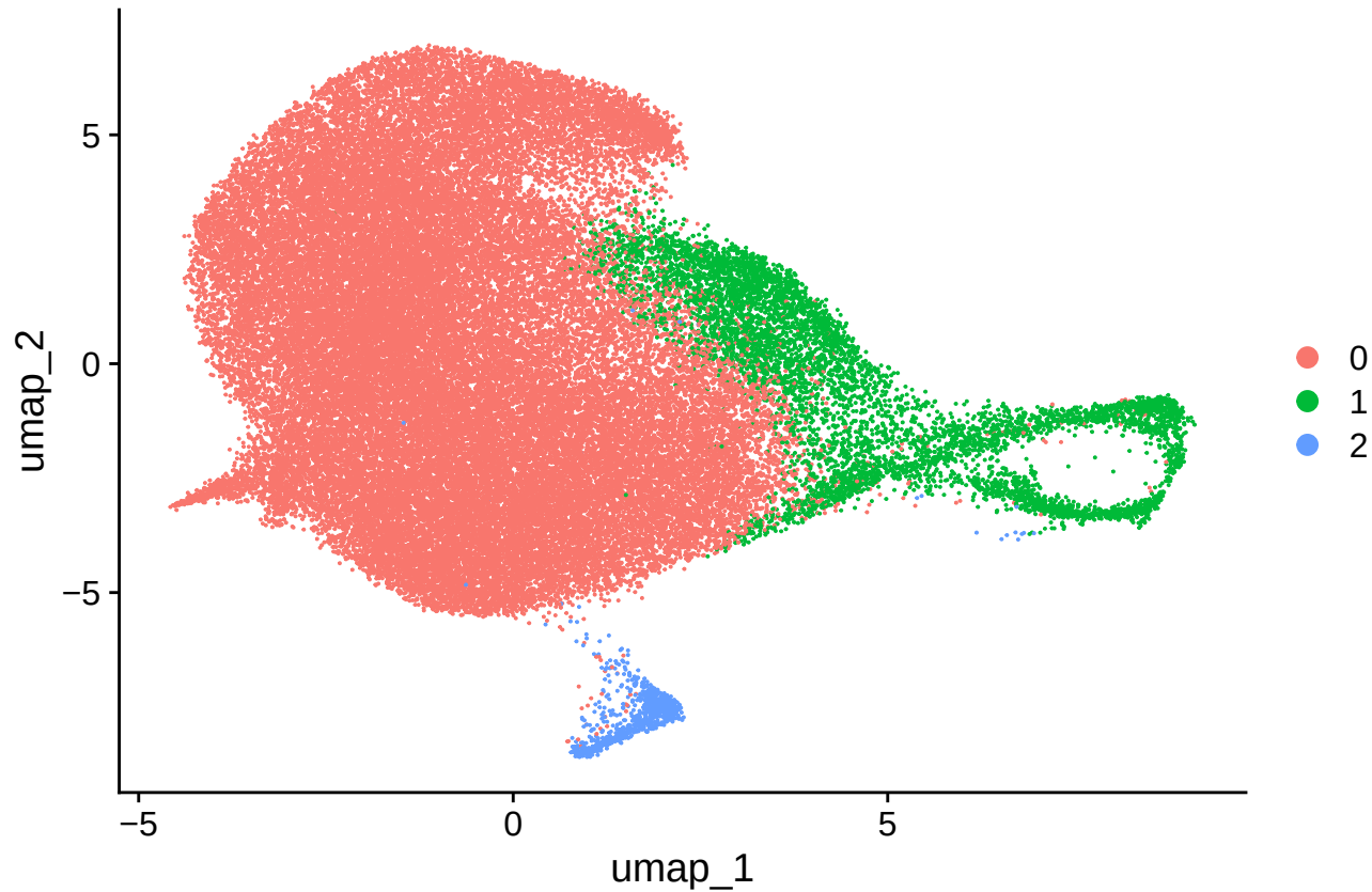
res0.1_clusters
