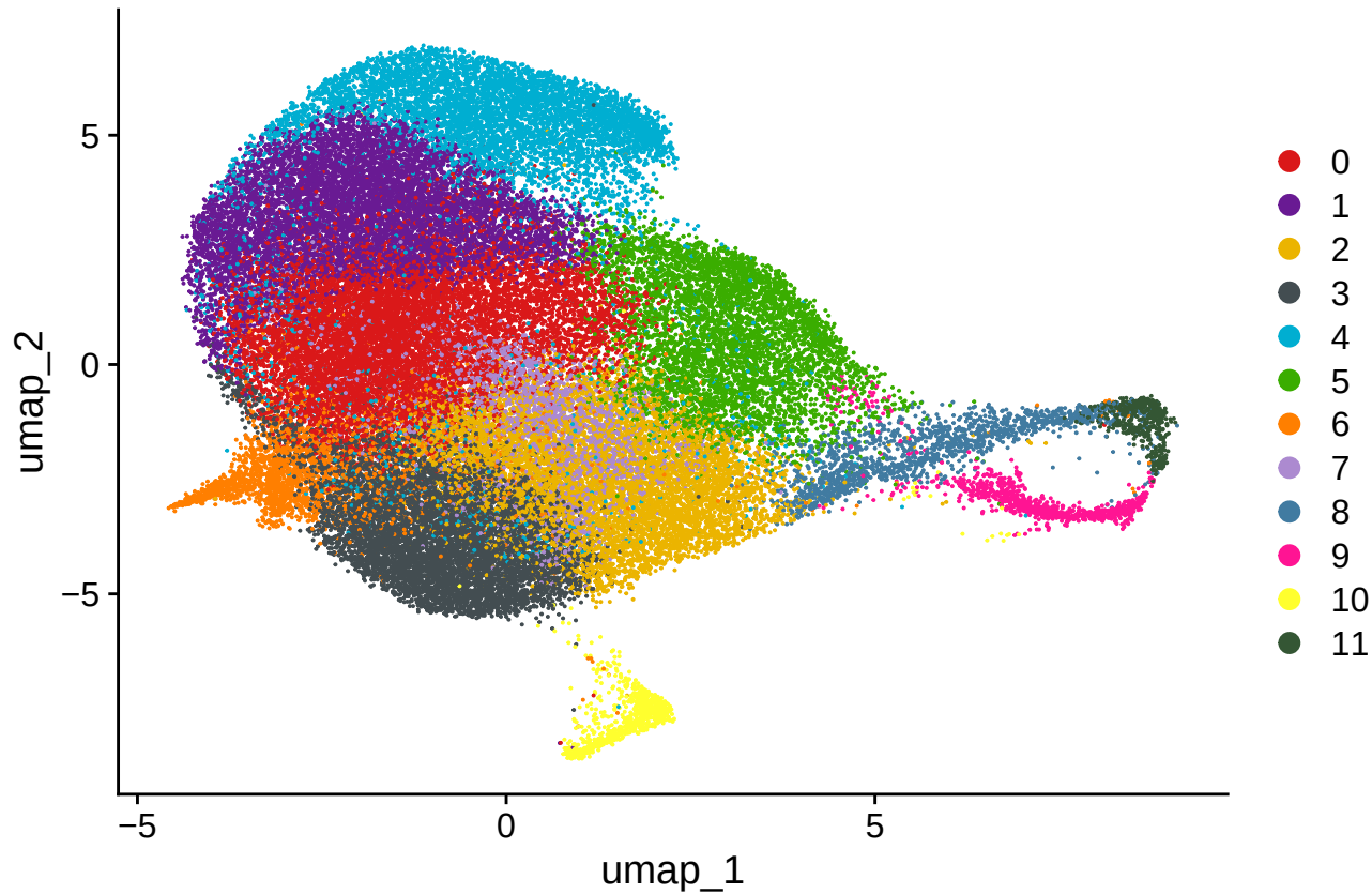
res0.5_clusters
