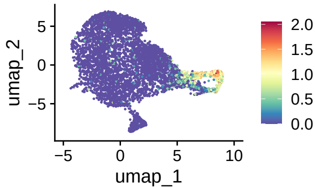
DTL
