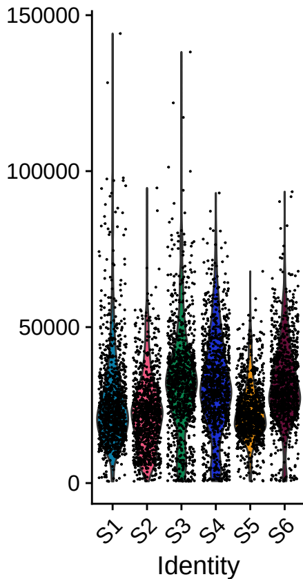
nCount_RNA
