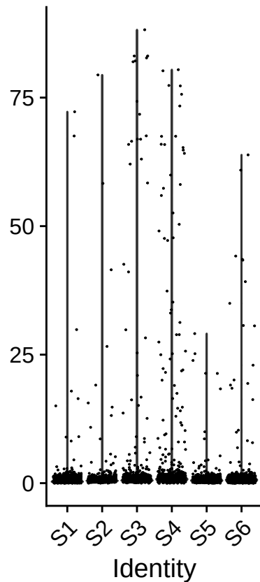
percent.mt
