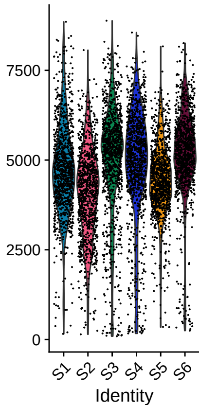
nFeature_RNA
