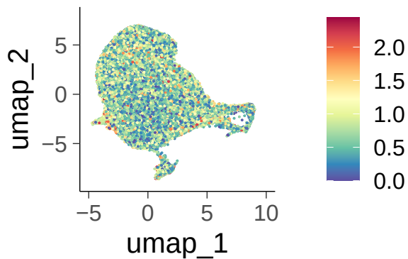
percent.mt
