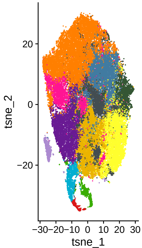
shc_clusters
