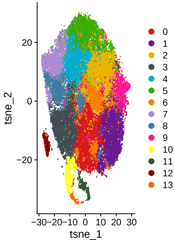
res0.8_clusters
