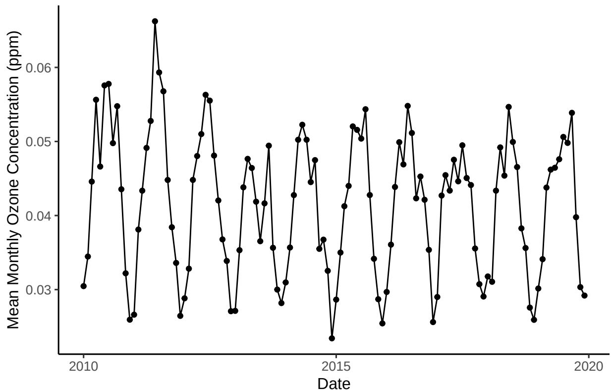
Mean Monthly Ozone Concentration From 2010 to 2019
