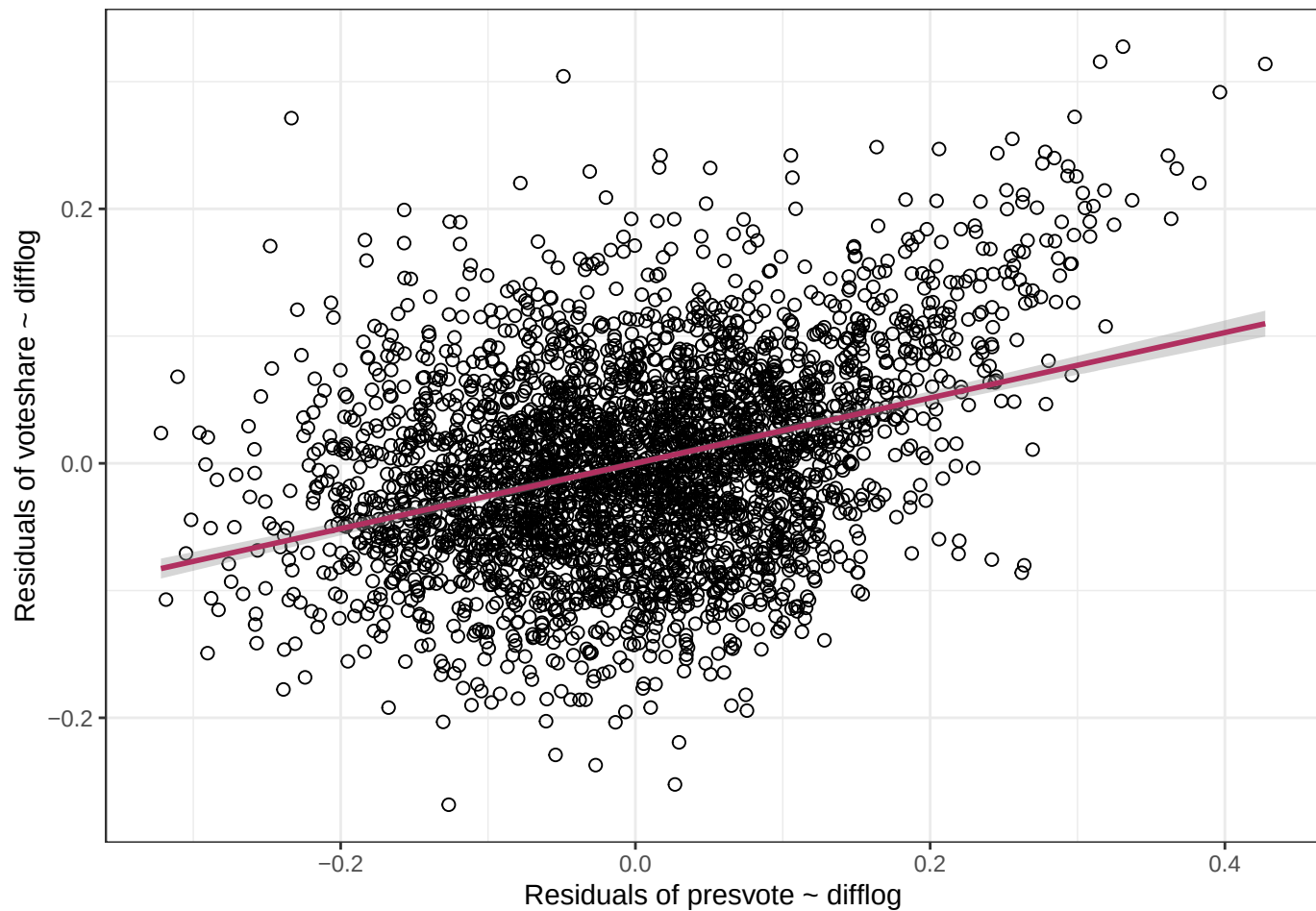
Residuals Regression: voteshare and presvote (Controlling for difflog)
