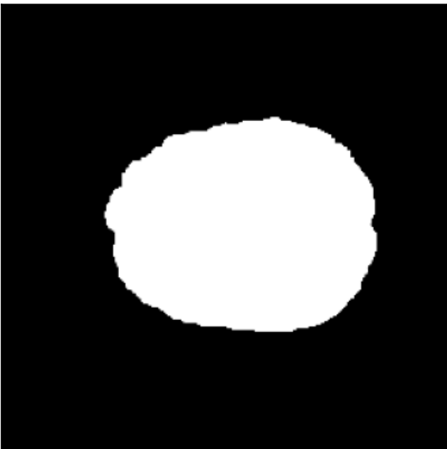
z = 0
