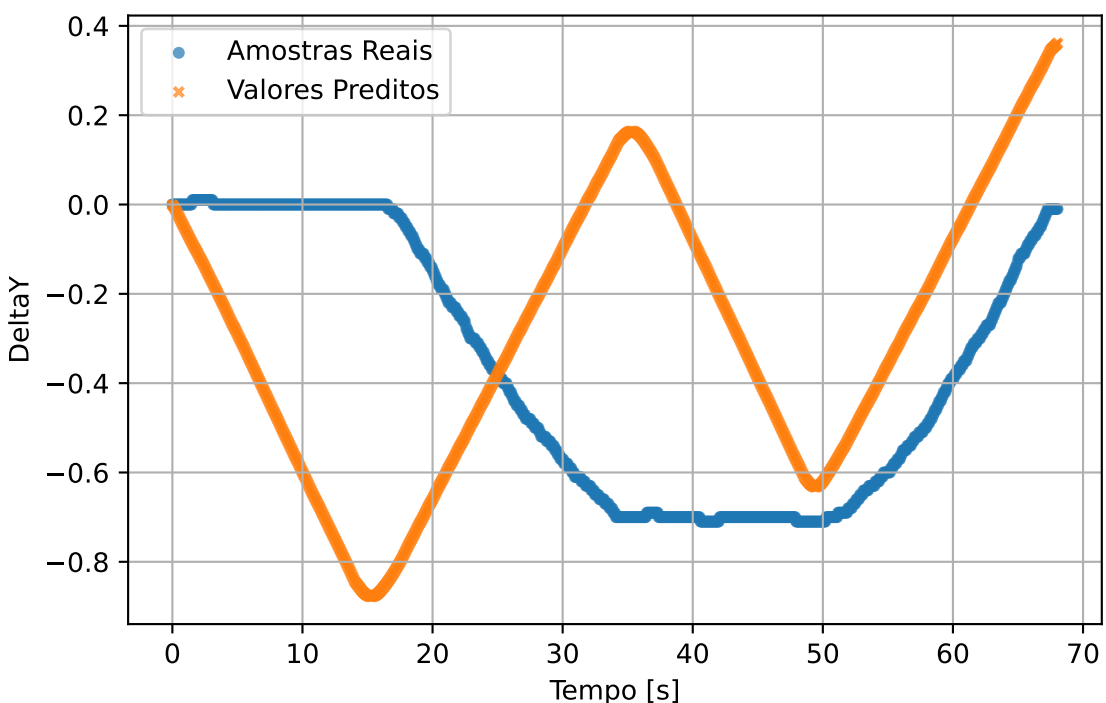
train2 - DeltaY
