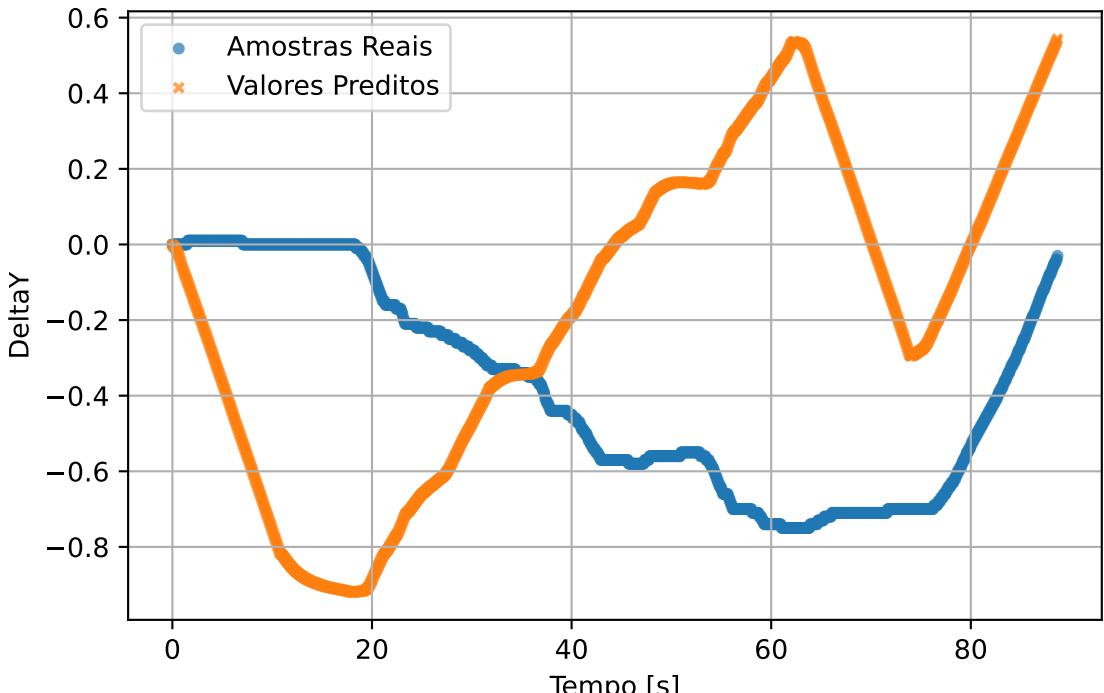
val - DeltaY
