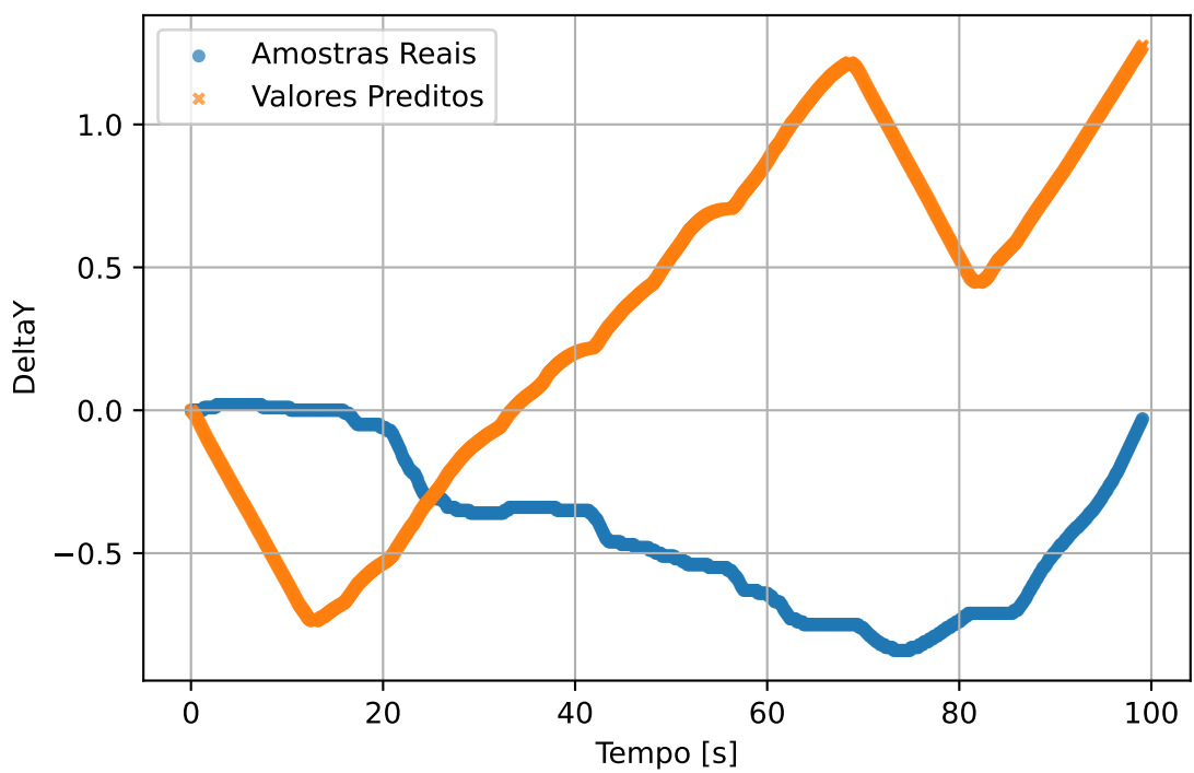
val - DeltaY
