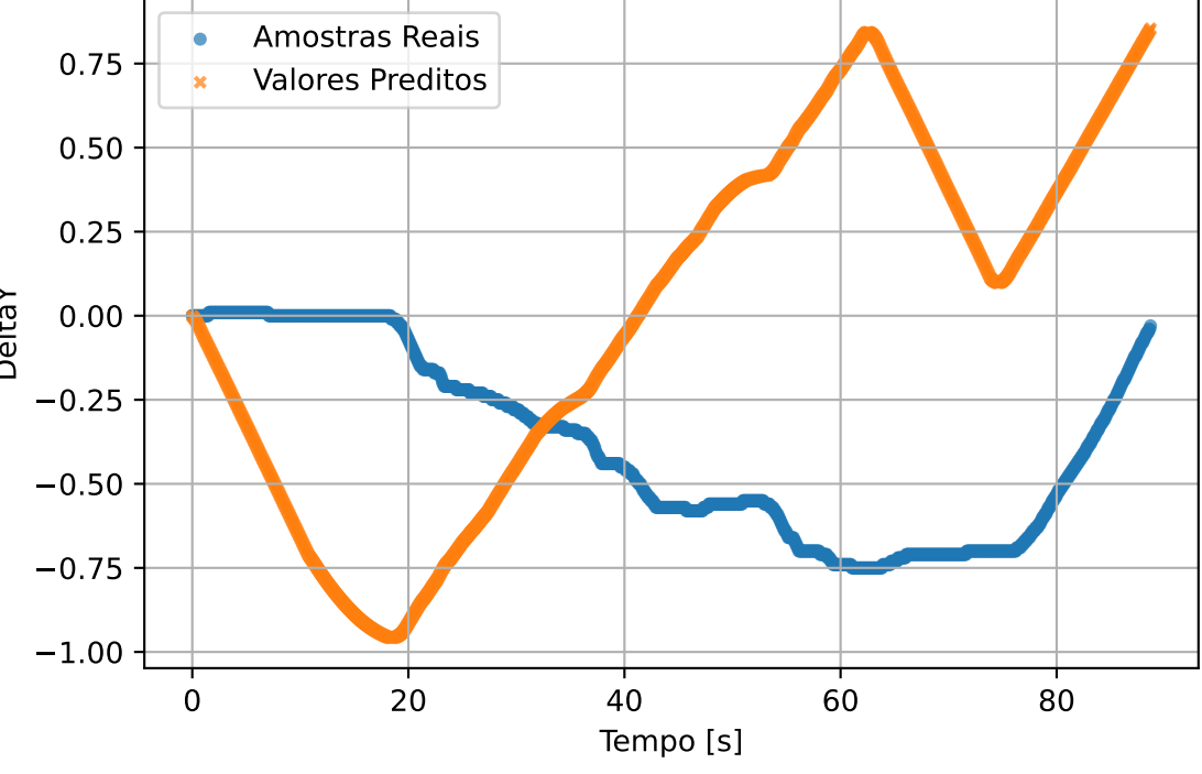
val - DeltaY
