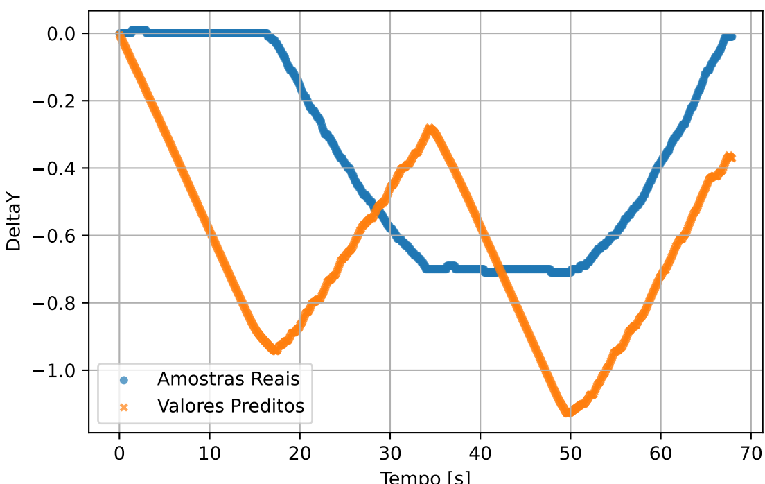
train2 - DeltaY
