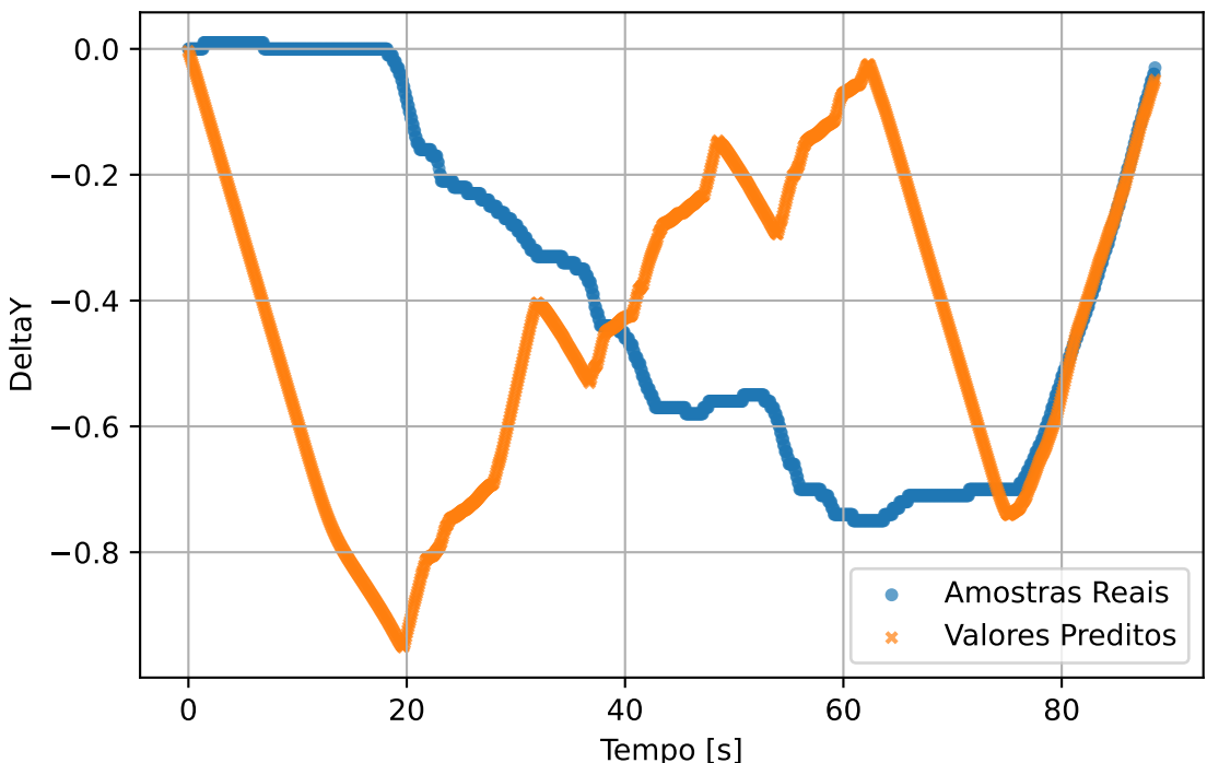
val - DeltaY
