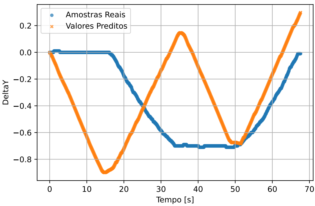
train2 - DeltaY
