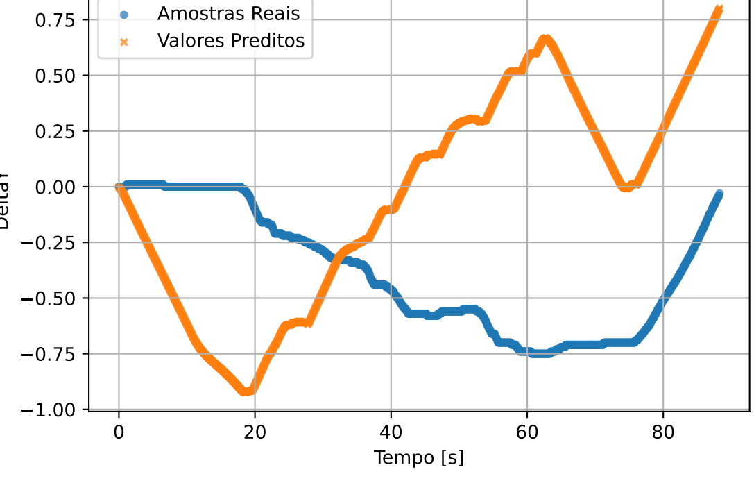
val - DeltaY
