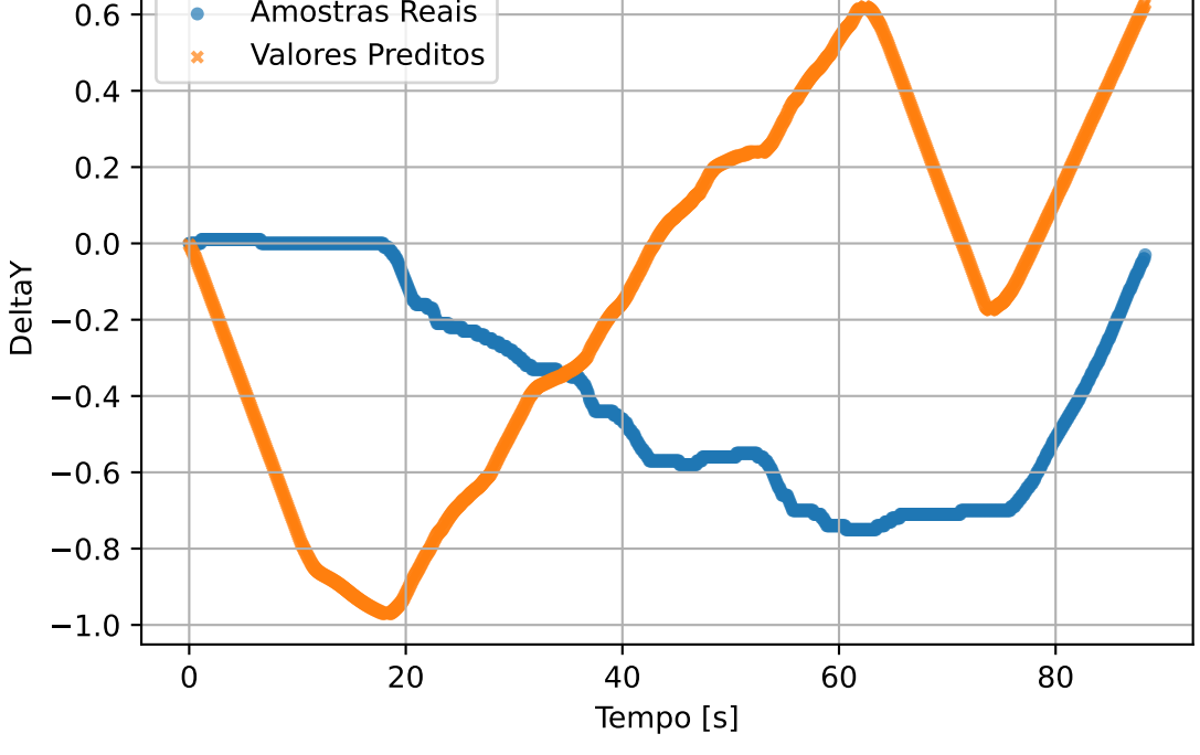
val - DeltaY
